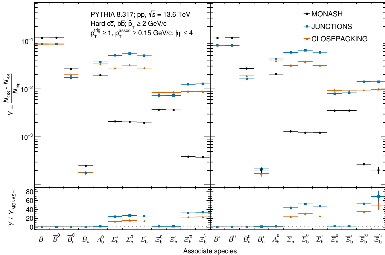
(b) \Lambda_b^0 trigger
