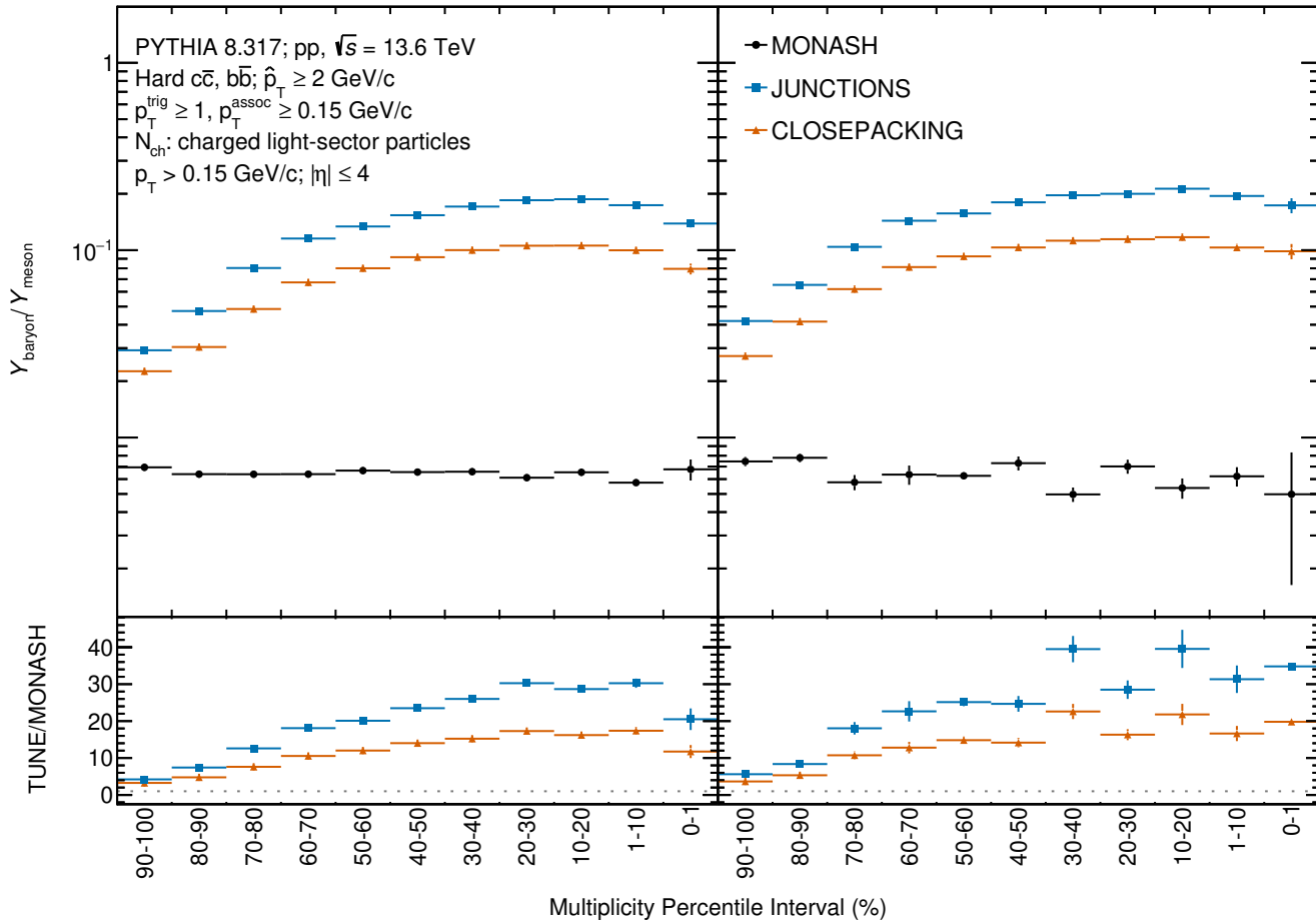
(a) D^0 trigger: \bar{\Sigma}_c^- / \bar{D}^0
