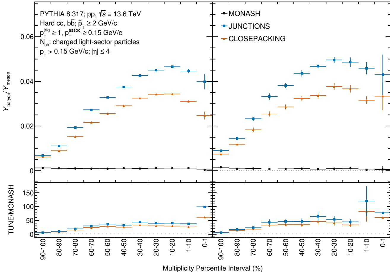
(a) D^0 trigger: \Xi_c^- / \bar{D}^0
