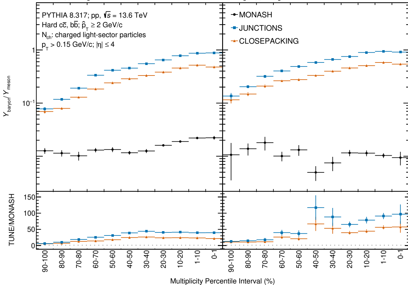
(a) B^+ trigger: \Sigma_b^0 / B^+
