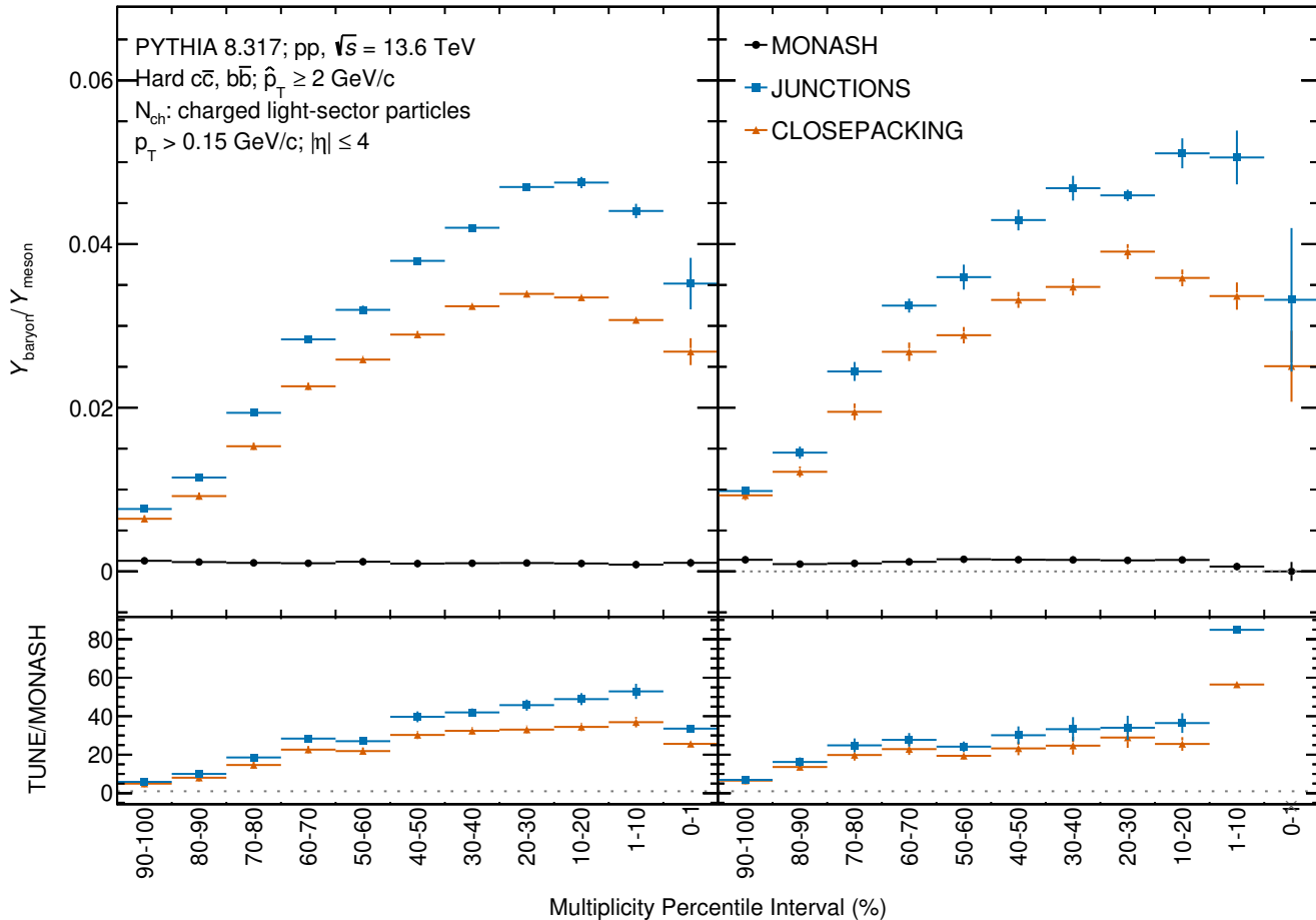
(a) D^0 trigger: \bar{\Xi}_c^0 / \bar{D}^0
