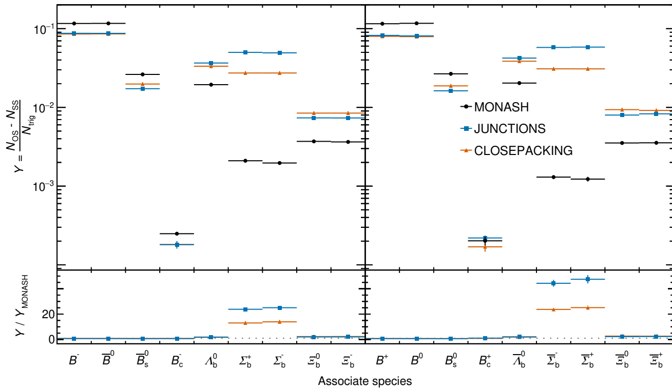
(b) \Lambda_b^0 trigger
