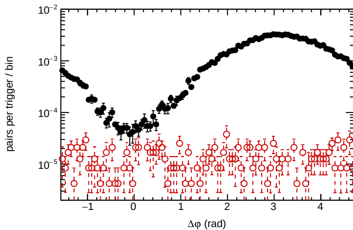
\bar{\Lambda}_b^0 trigger
