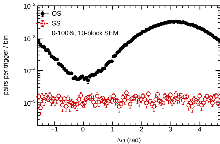
B^+ trigger
