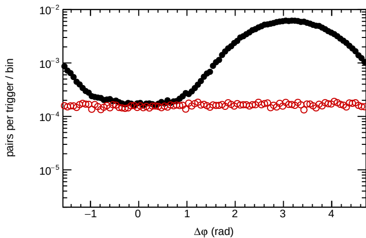
\Lambda_c^+ trigger
