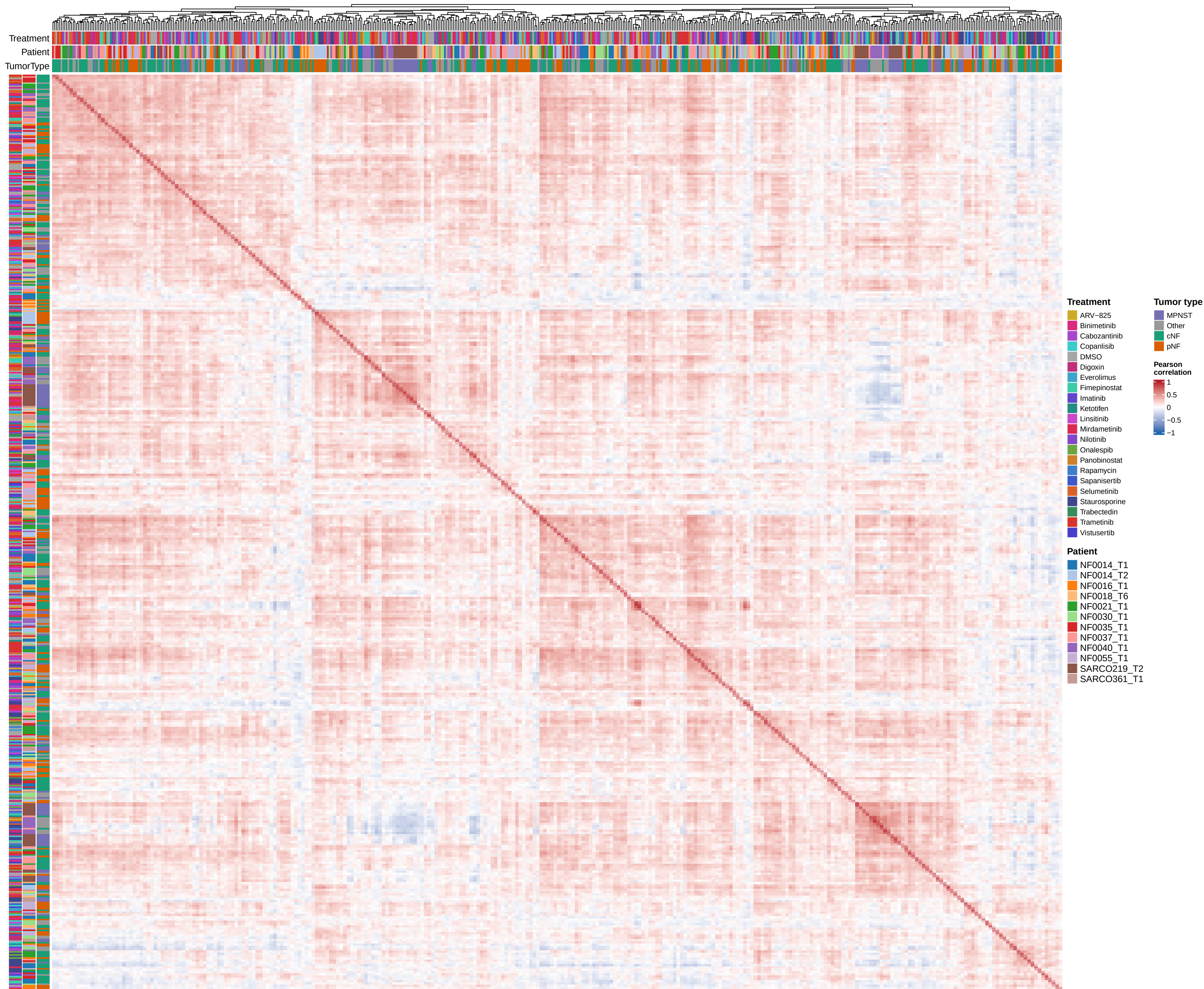
2D Middle Slice ... Single-Cell Aggregate Profiles ... Replicate Correlation (Clustered)
