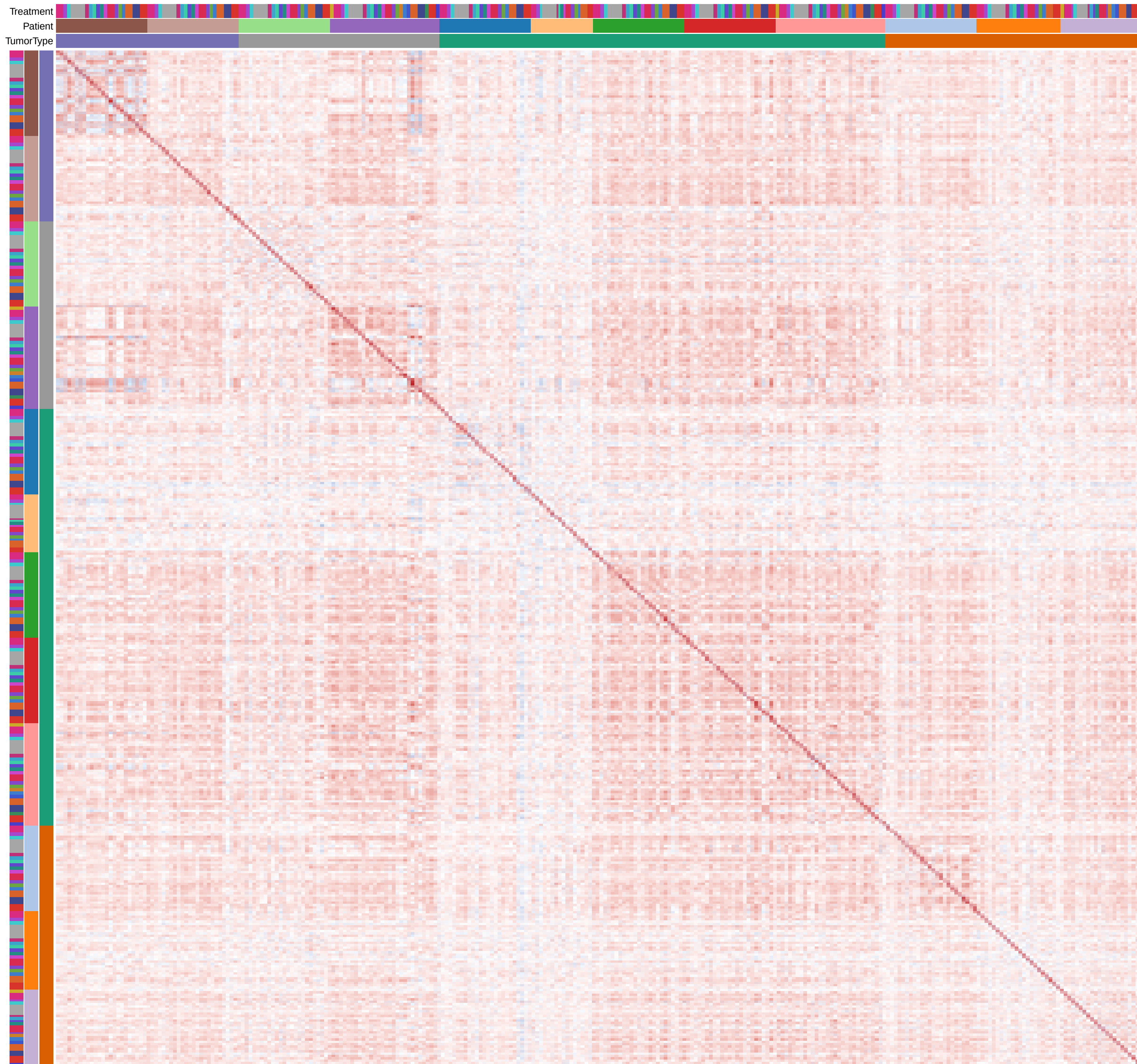
2D Middle Slice ... Single-Cell Aggregate Profiles ... Replicate Correlation (Unclustered)
