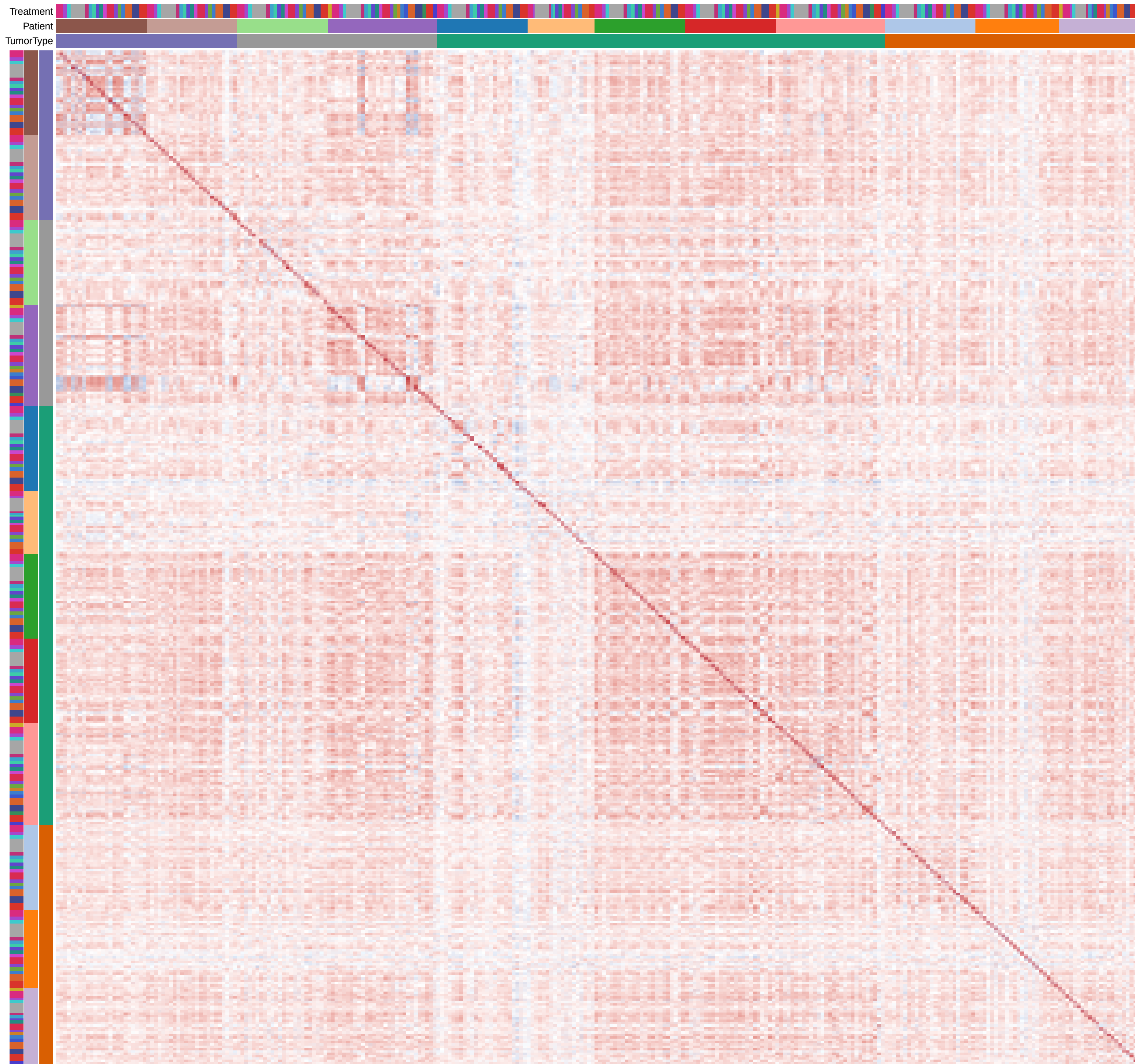
2D Middle N Slice ... Single-Cell Aggregate Profiles ... Replicate Correlation (Unclustered)
