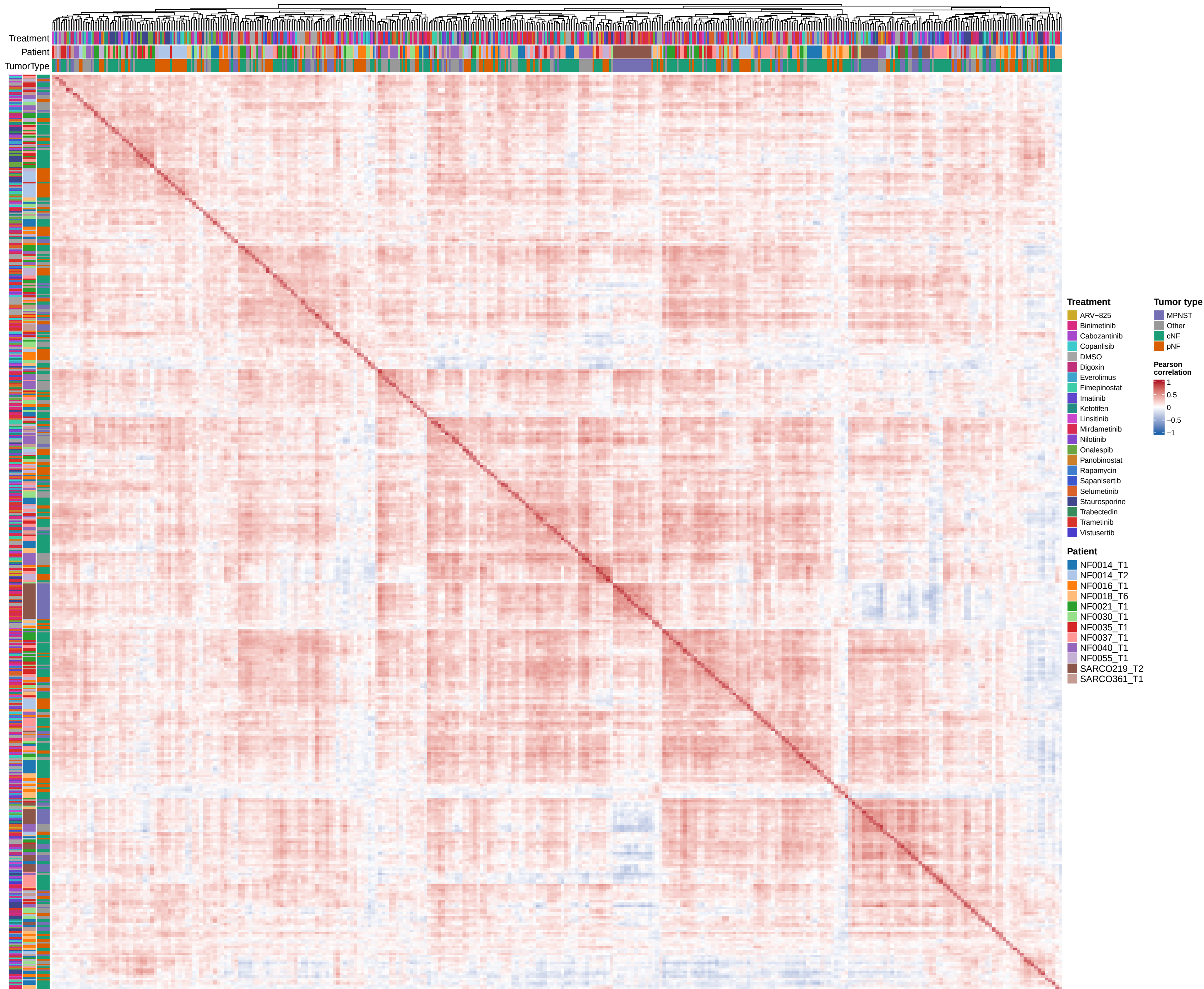
2D Middle N Slice ... Single-Cell Aggregate Profiles ... Replicate Correlation (Clustered)
