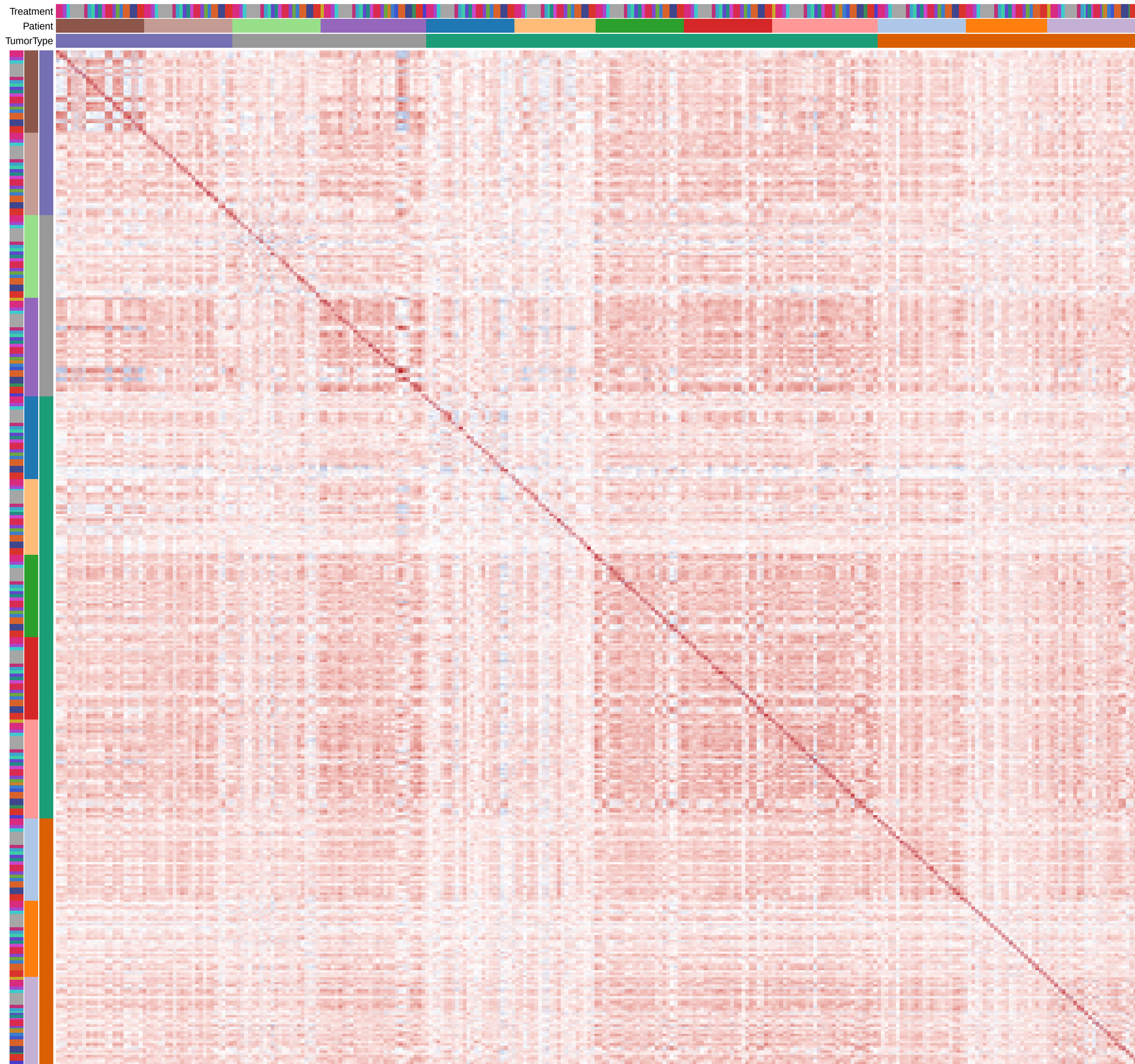
2D Max Projection ... Single-Cell Aggregate Profiles ... Replicate Correlation (Unclassified)
