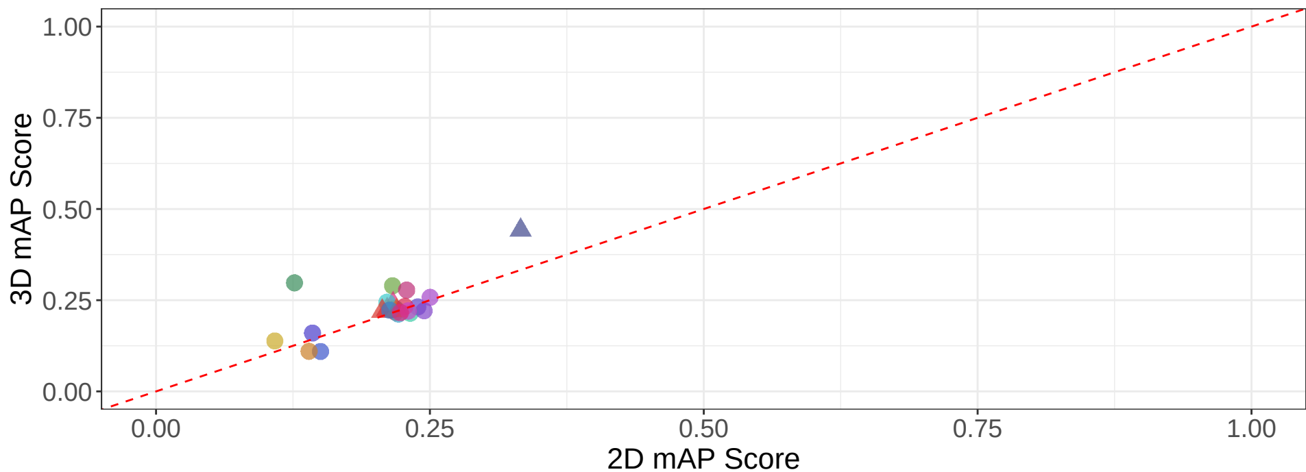
2D vs 3D Inter-patient mAP – Organoid – Handcrafted
