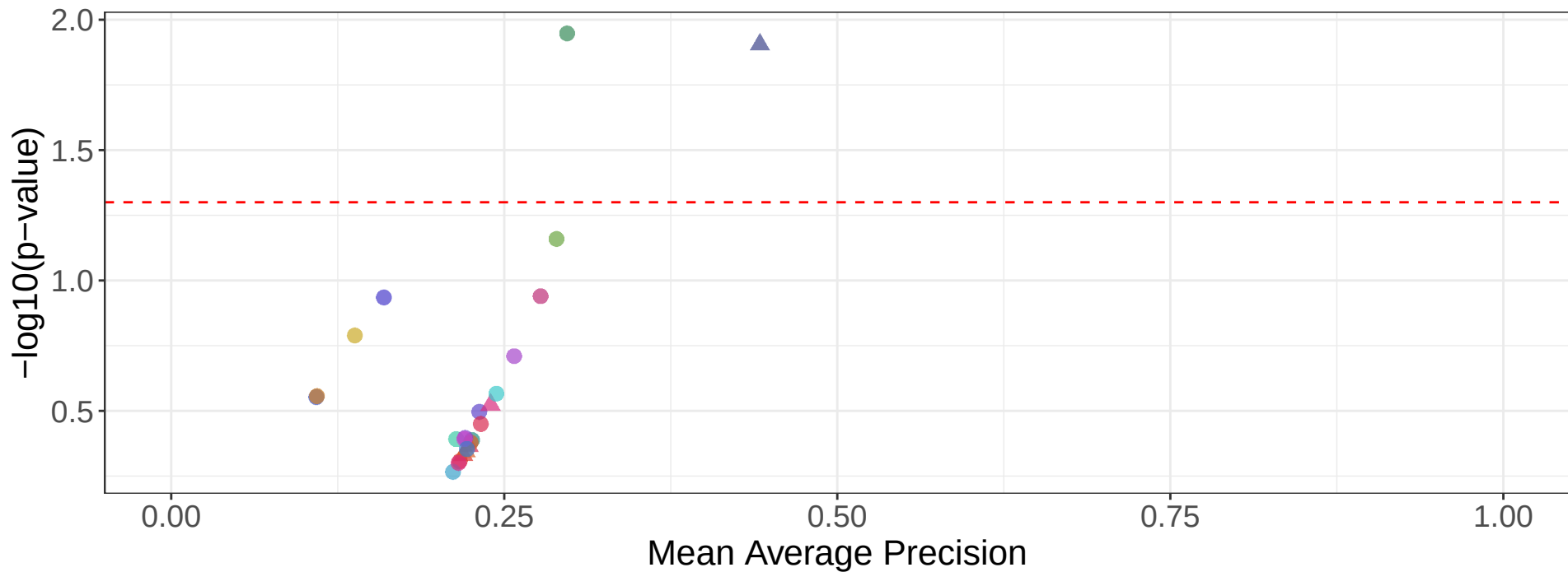
Inter-patient mAP – 3D Organoid – Handcrafted
