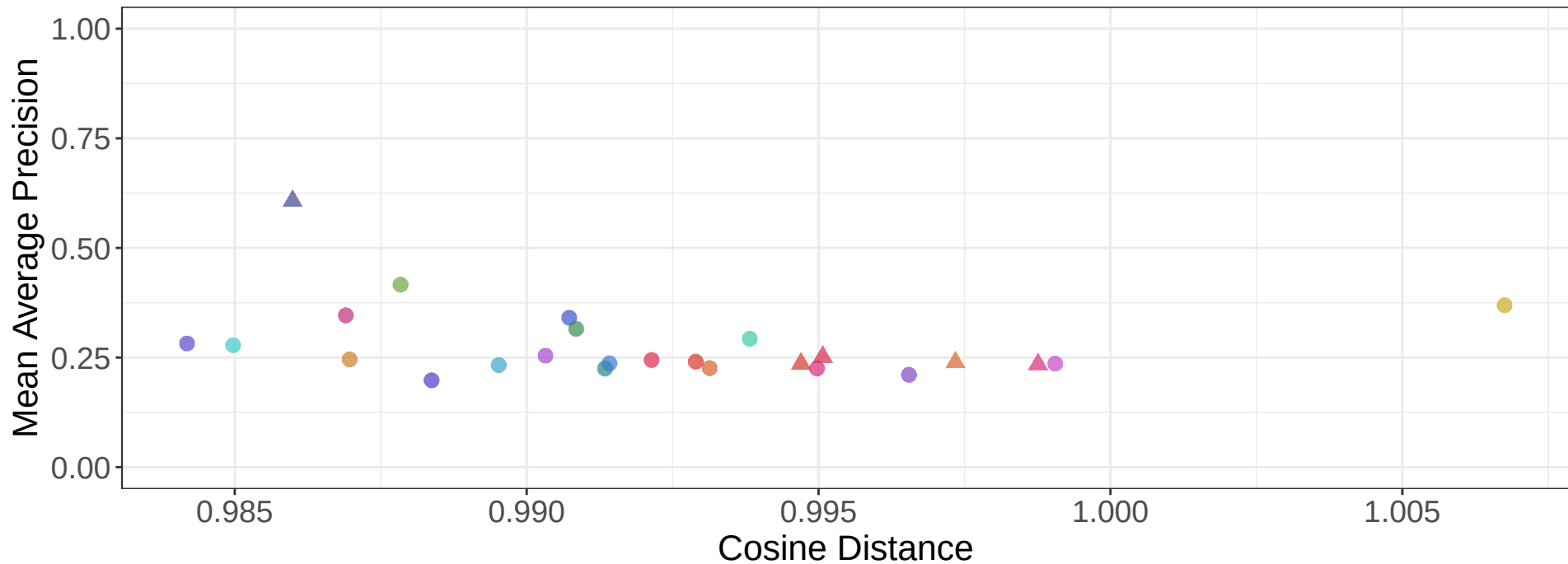
Inter-patient mAP vs Distance – 3D Single-cell – Nucleocentric DL (SAM-Med3D)
