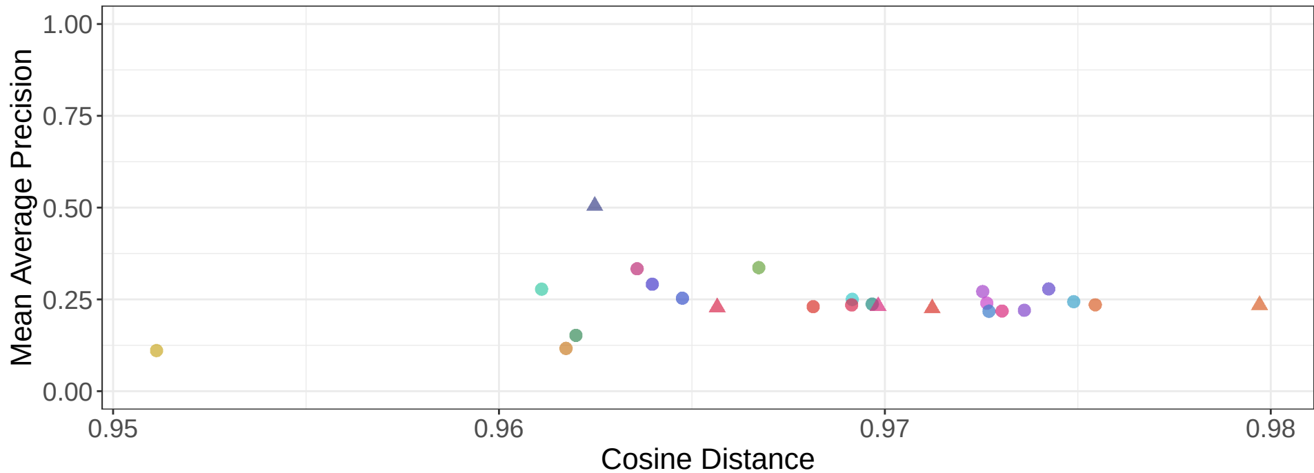
Inter-patient mAP vs Distance – 3D Single-cell – Handcrafted
