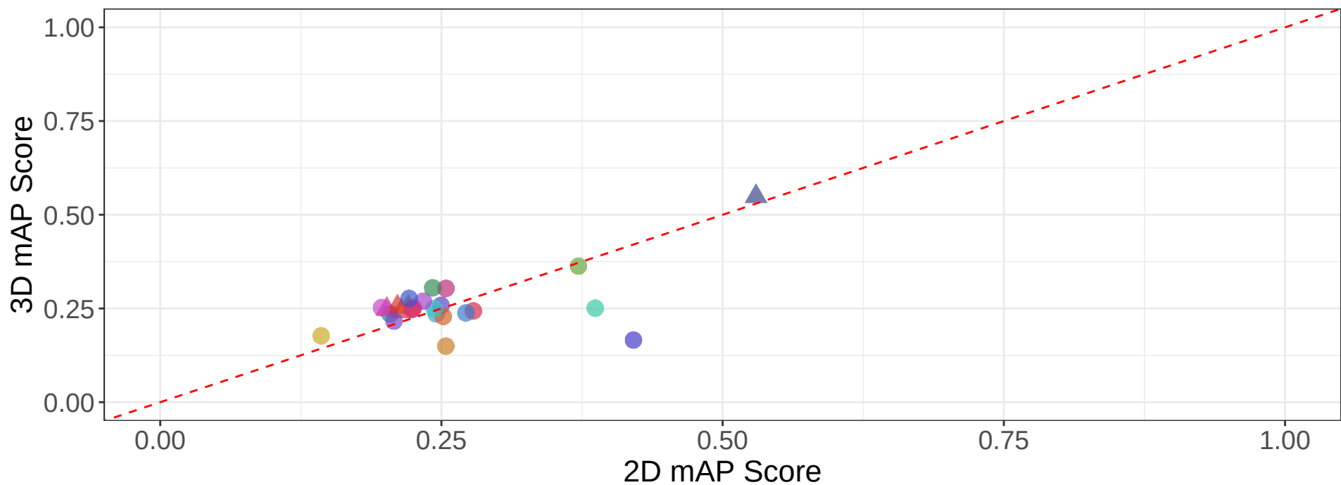
2D vs 3D Inter-patient mAP – Single-cell – DL (SAM-Med3D)
