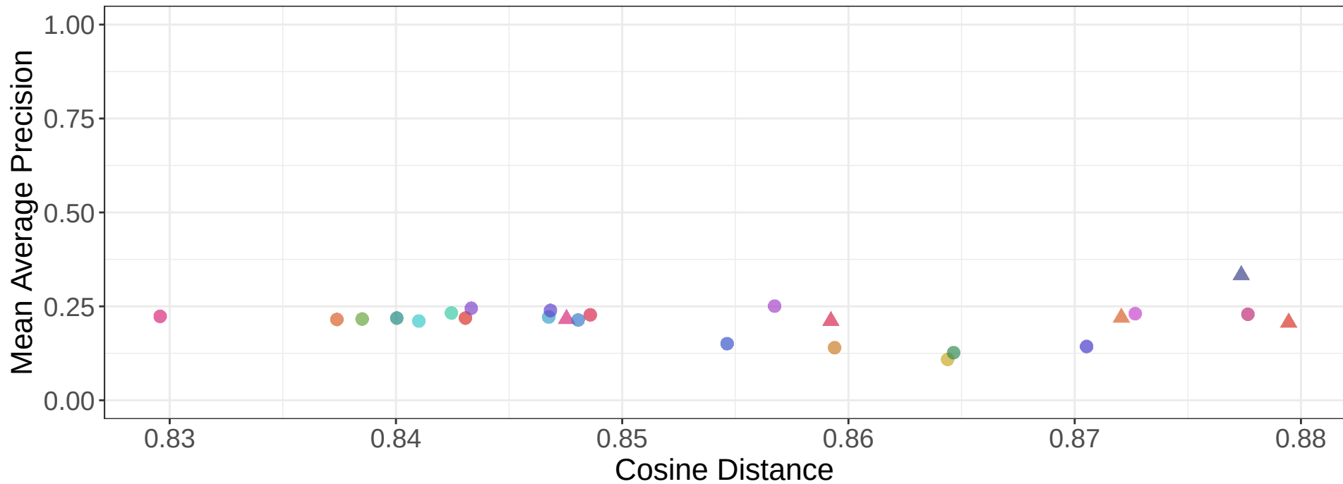
Inter-patient mAP vs Distance – 2D Organoid
