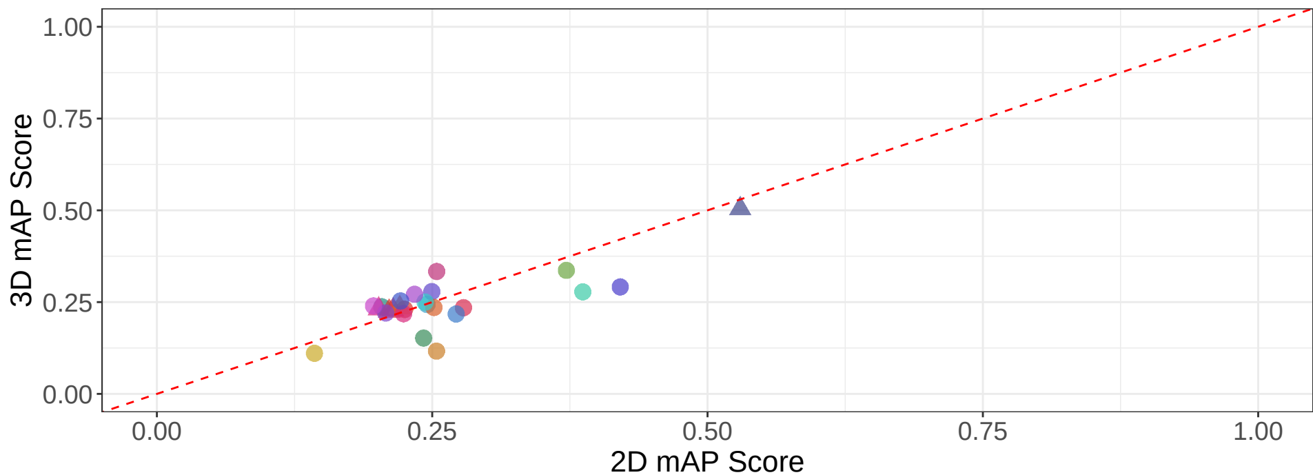
2D vs 3D Inter-patient mAP – Single-cell – Handcrafted
