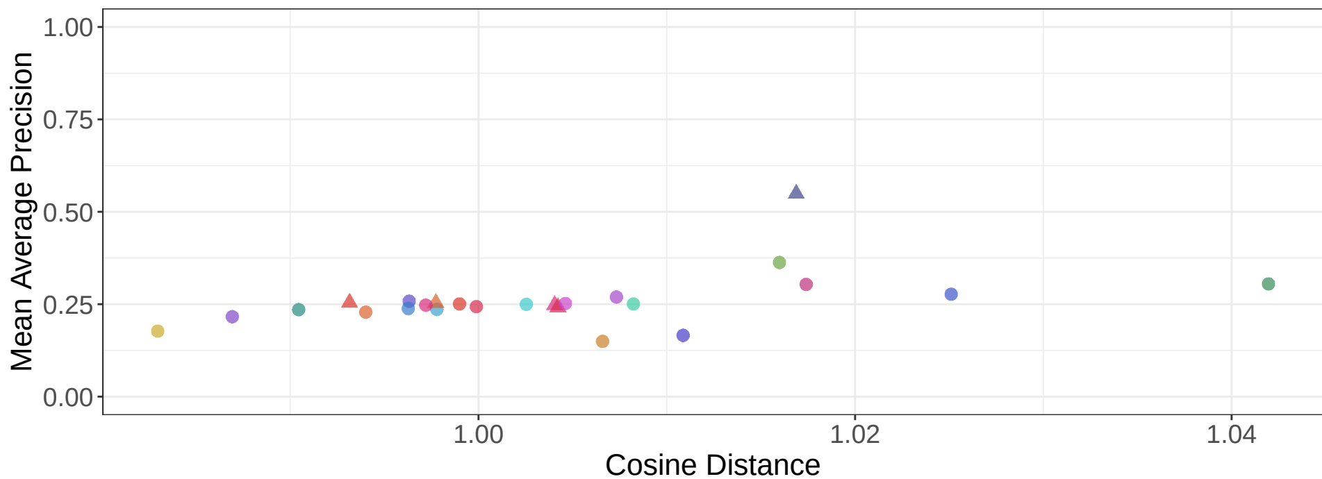
Inter-patient mAP vs Distance – 3D Single-cell – DL (SAM-Med3D)
