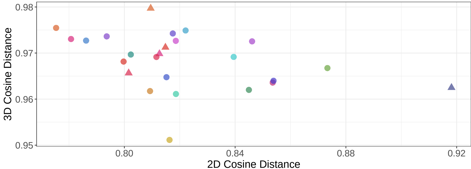
2D vs 3D Inter-patient Cosine Distance – Single-cell – Handcrafted
