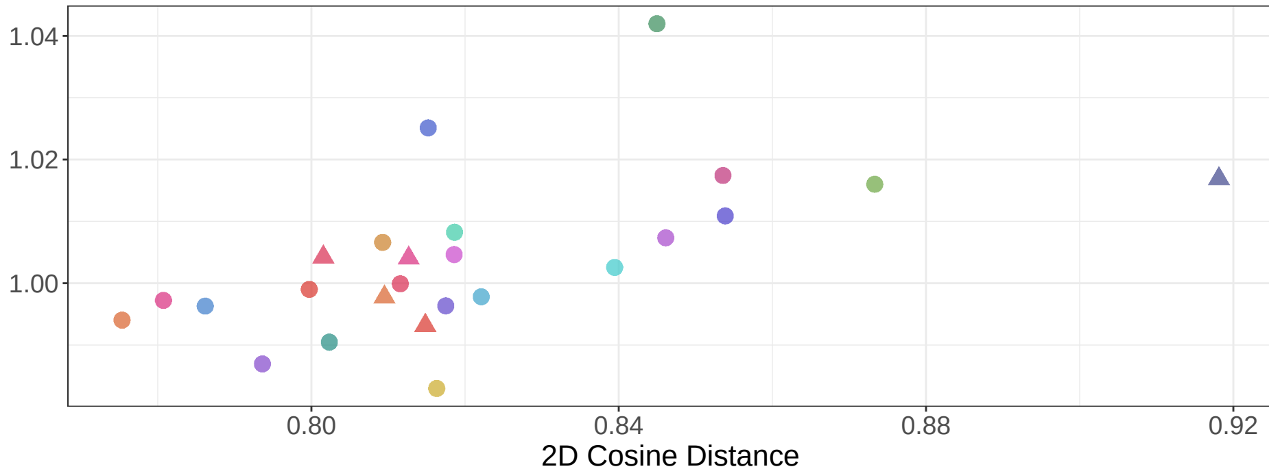
2D vs 3D Inter-patient Cosine Distance – Single-cell – DL (SAM-Med3D)
