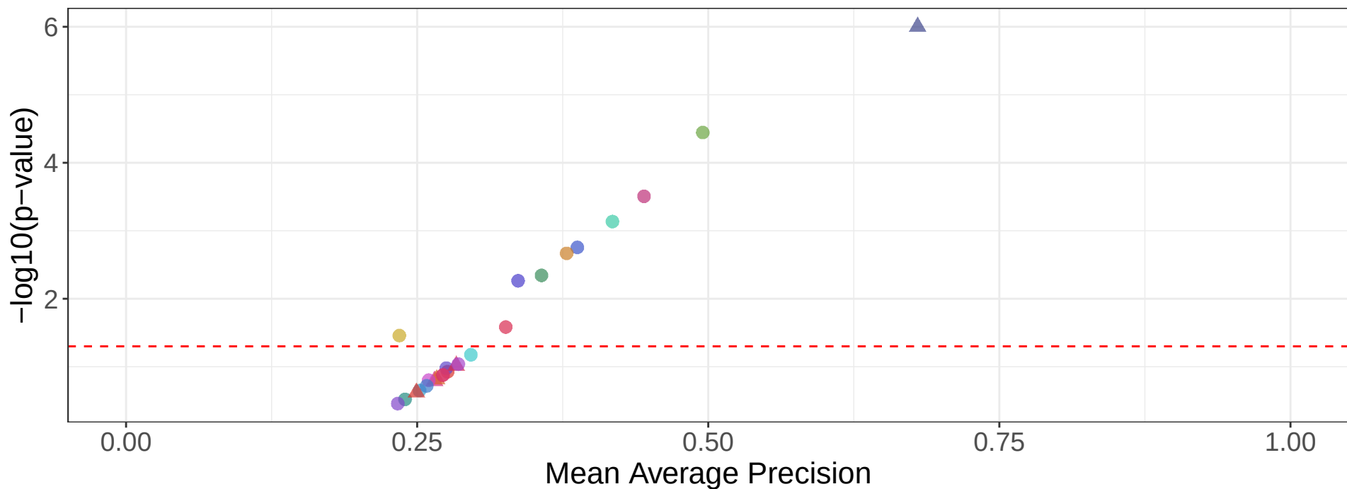
Inter-patient mAP – 3D Single-cell – Nucleocentric DL (MorphEM)
