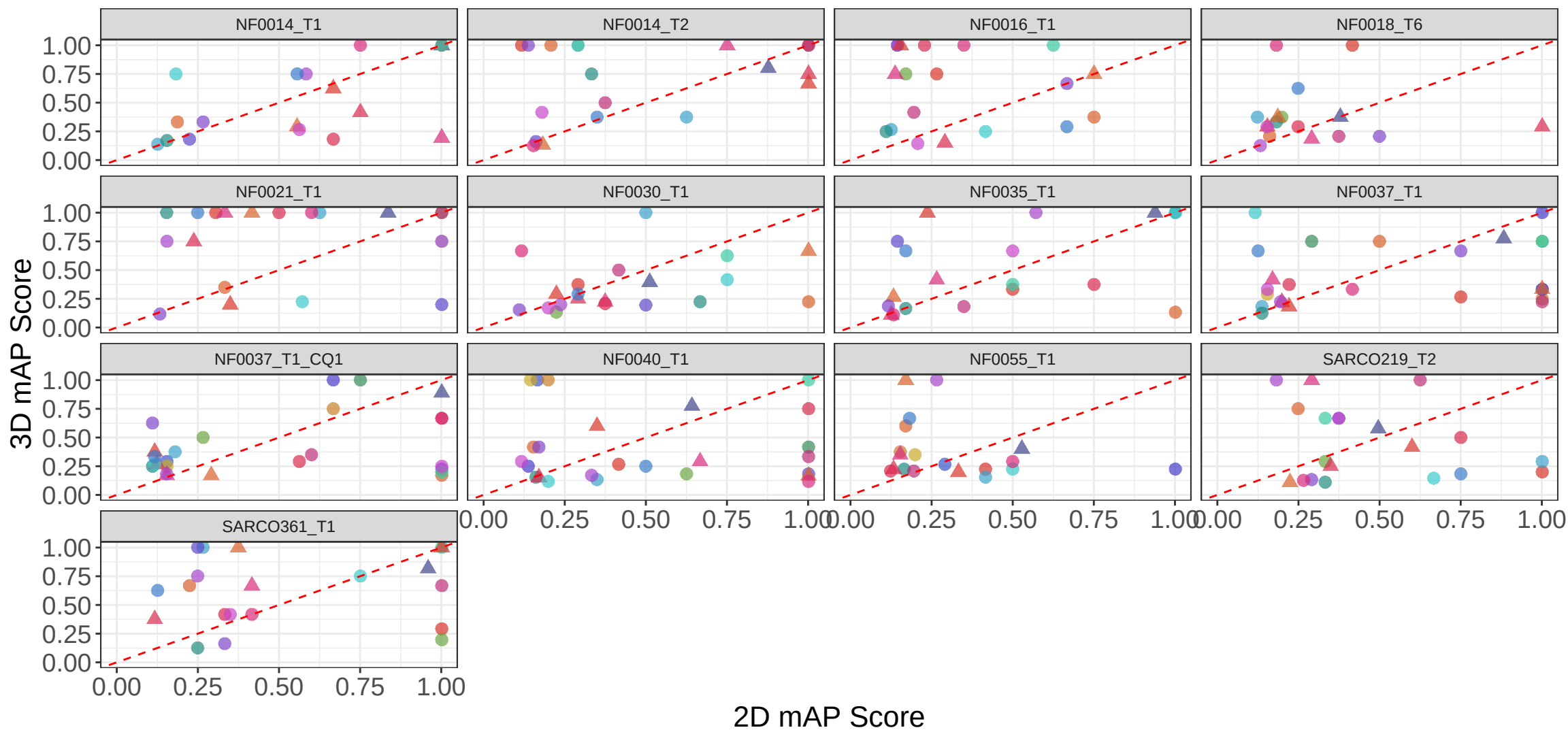
2D vs 3D Intra-patient mAP – Single-cell – DL (SAM-Med3D)
