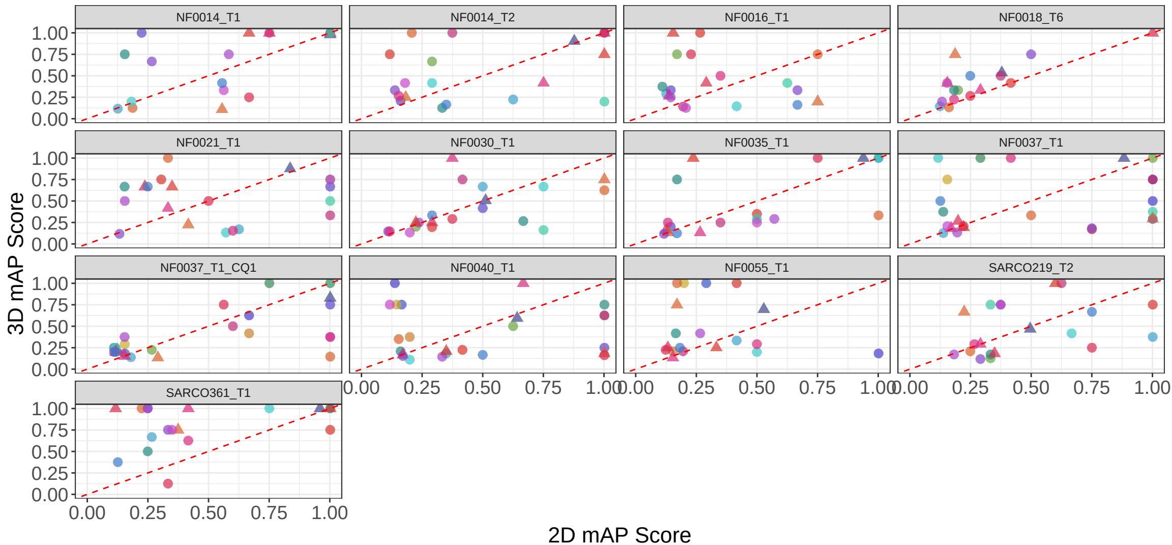
2D vs 3D Intra-patient mAP – Single-cell – Nucleocentric DL (SAM-Med3D)
