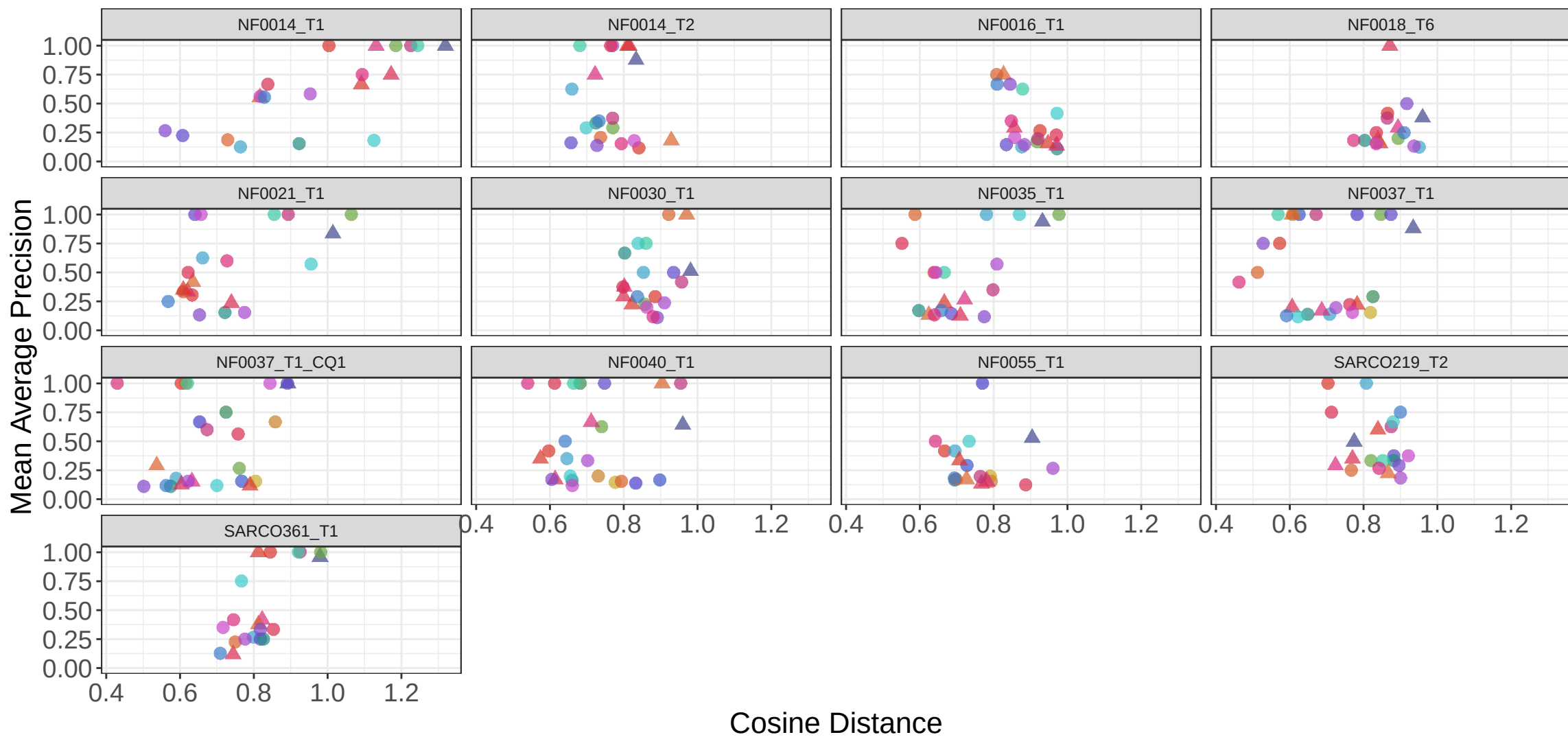
Intra-patient mAP vs Distance – 2D Single-cell
