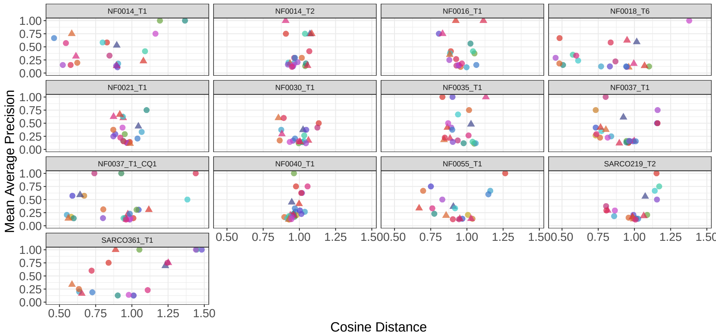
Intra-patient mAP vs Distance – 3D Organoid – DL (SAM–Med3D)
