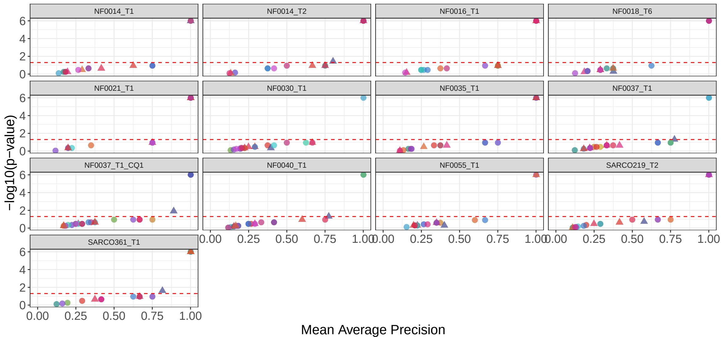
Intra-patient mAP – 3D Single-cell – DL (SAM-Med3D)
