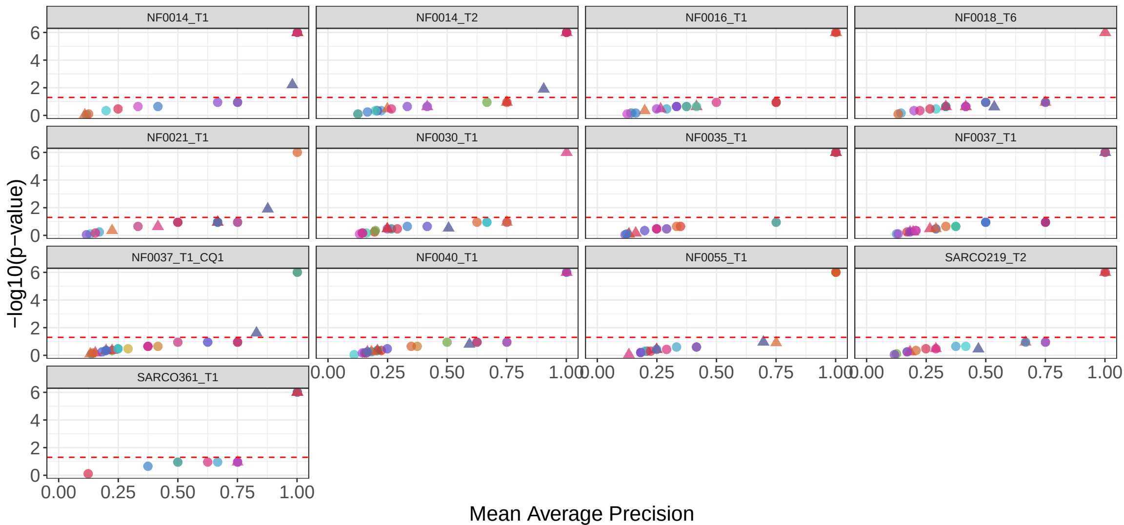
Intra-patient mAP – 3D Single-cell – Nucleocentric DL (SAM-Med3D)
