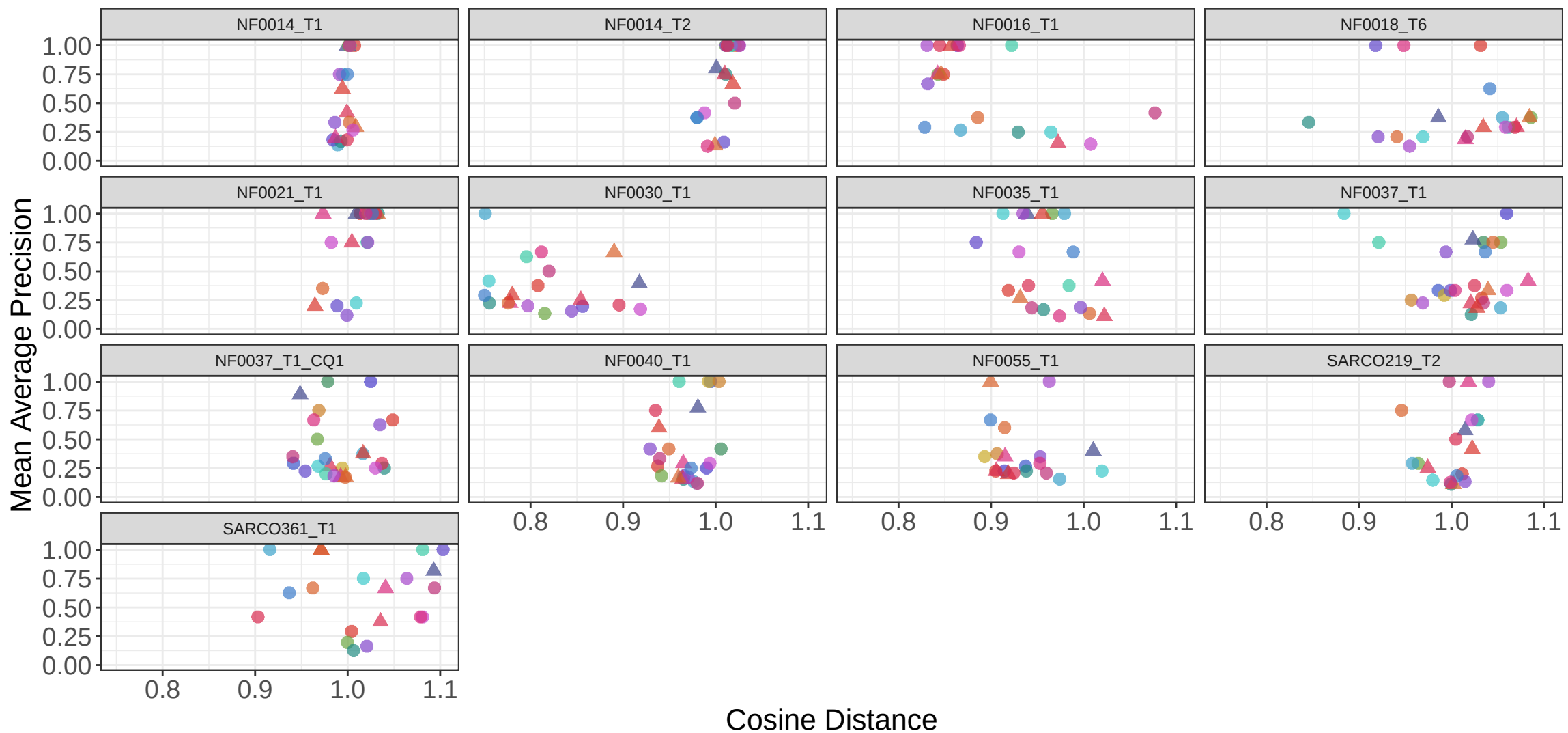
Intra-patient mAP vs Distance – 3D Single-cell – DL (SAM-Med3D)
