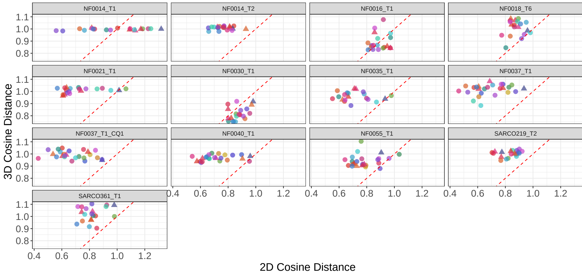
2D vs 3D Intra-patient Cosine Distance – Single-cell – DL (SAM-Med3D)
