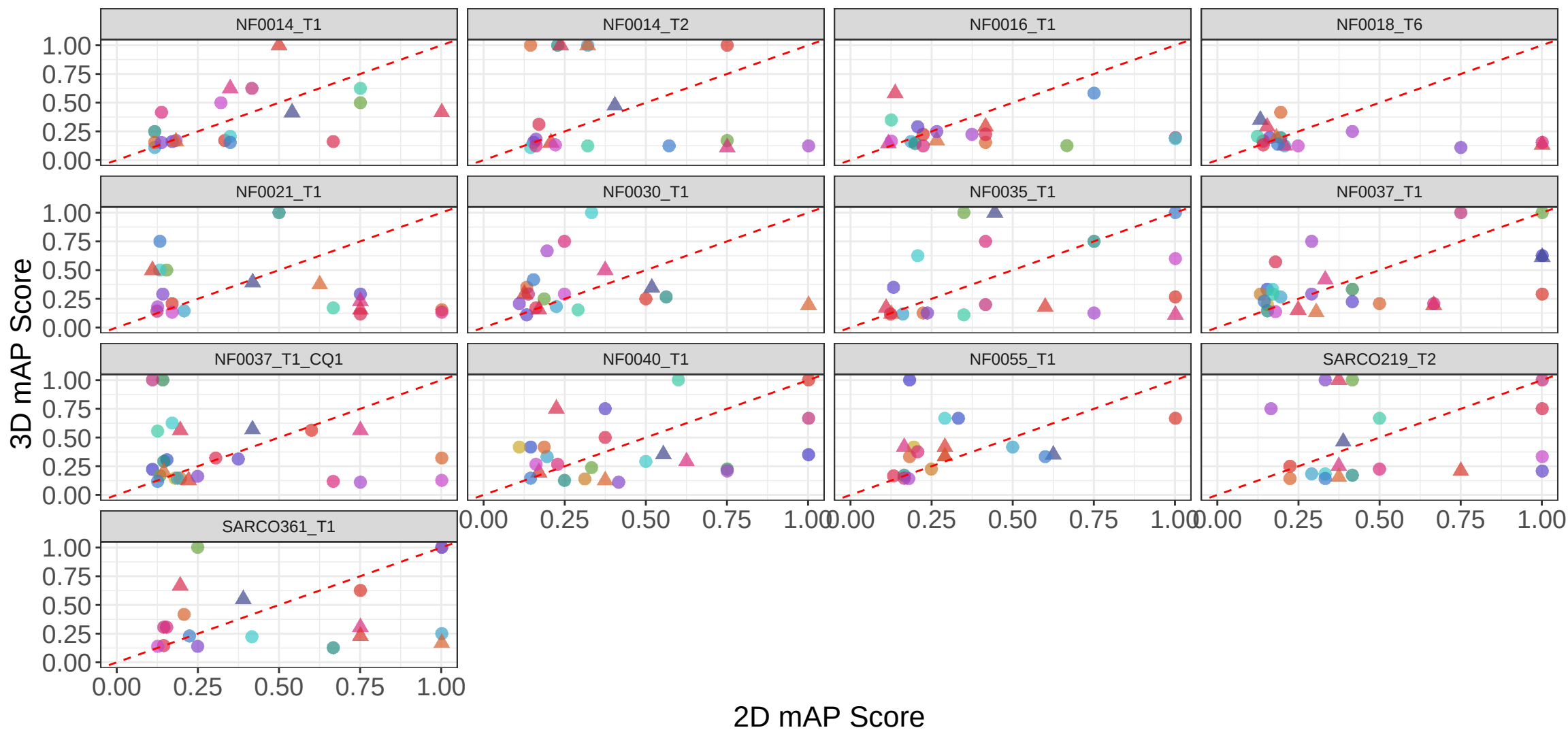
2D vs 3D Intra-patient mAP – Organoid – Handcrafted
