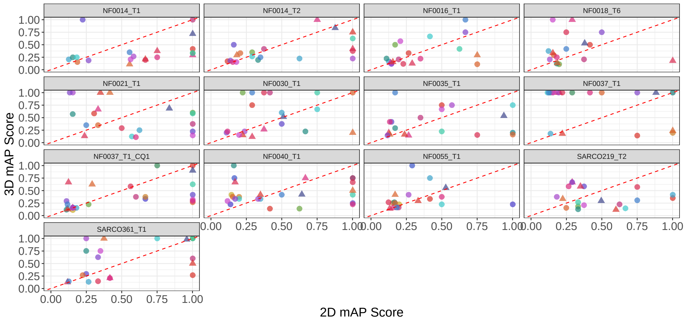
2D vs 3D Intra-patient mAP – Single-cell – Handcrafted
