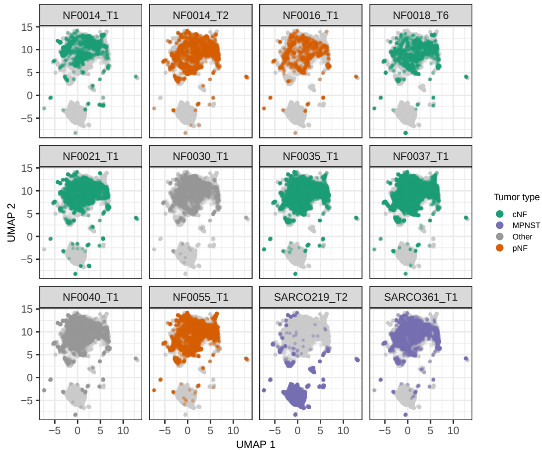
All patients: 3D Single Cell FS Profiles
