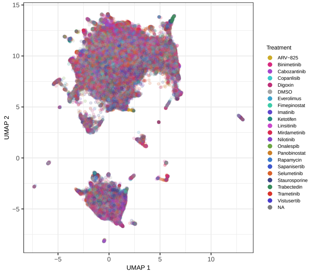
All patients: 3D Single Cell FS Profiles
