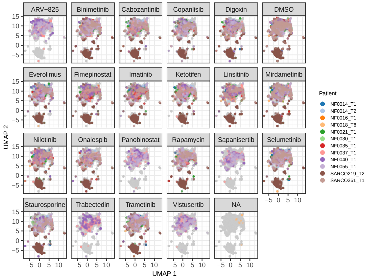
All patients: 3D Single Cell FS Profiles
