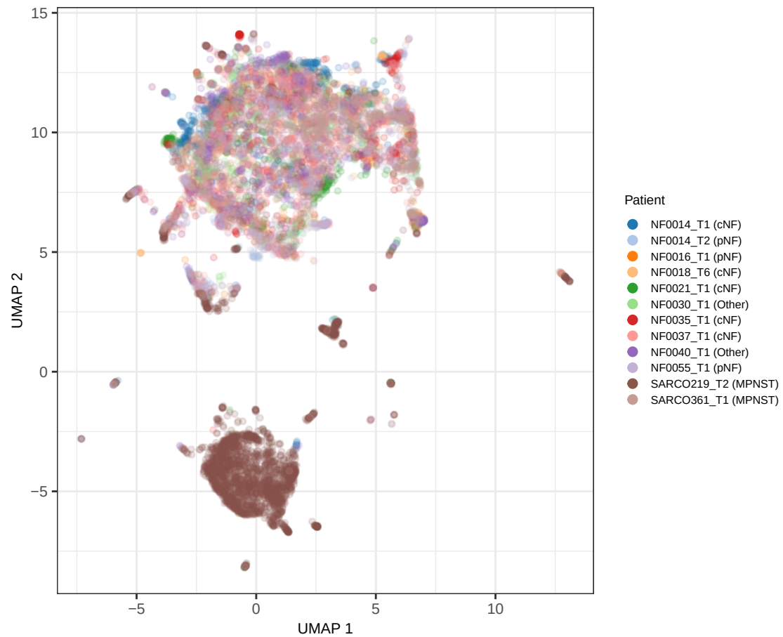
All patients: 3D Single Cell FS Profiles (DMSO Controls)
