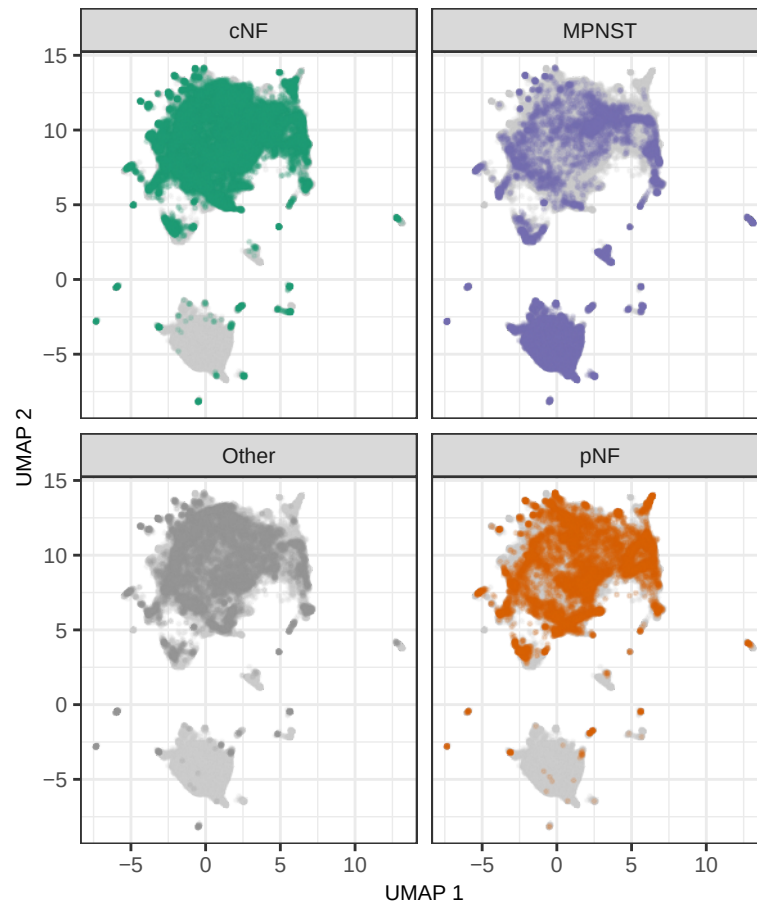
All patients: 3D Single Cell FS Profiles
