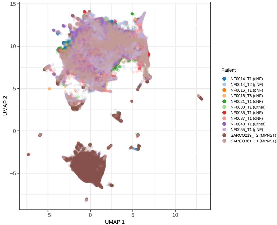
All patients: 3D Single Cell FS Profiles
