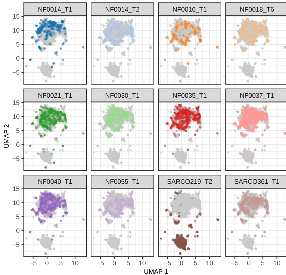
All patients: 3D Single Cell FS Profiles (DMSO Controls)
