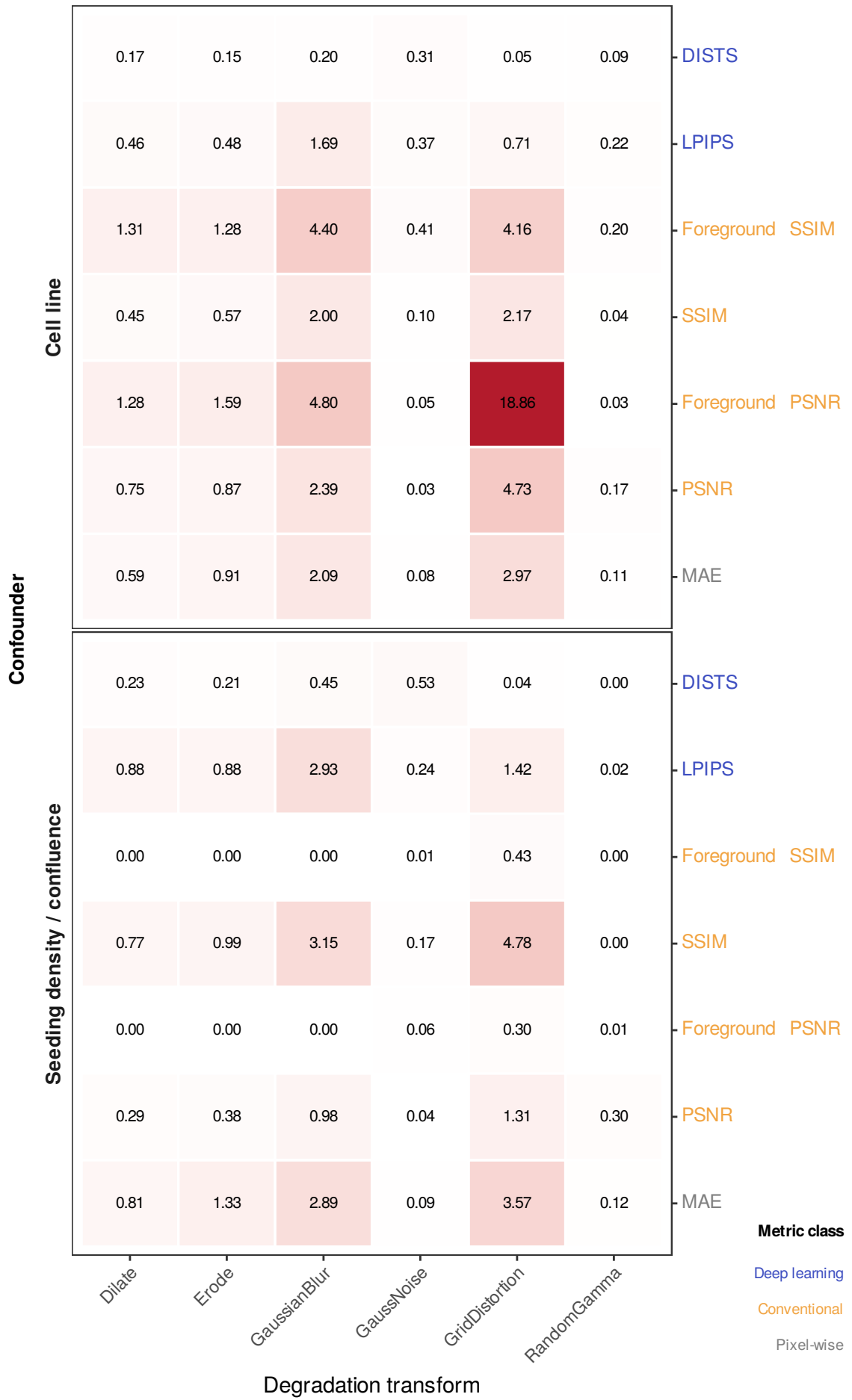
Burden (partial R^2 / restricted R^2)
