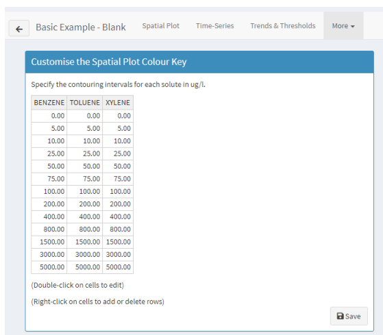
Figure 19: Customising the Spatial plot Colour Key.
