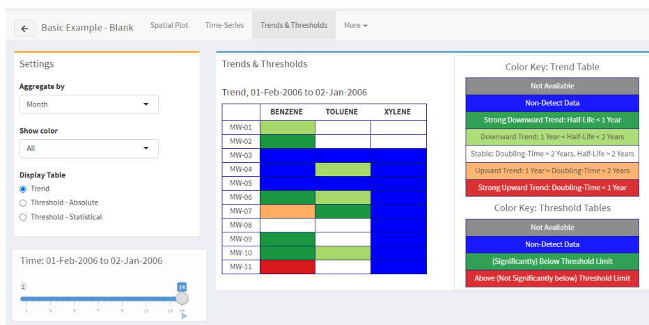
Figure 16: GWSDAT Trends and Thresholds plot.
