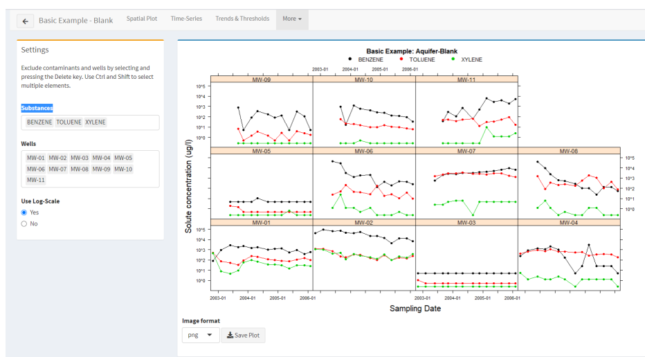
Figure 17: GWSDAT Well Report plot.
