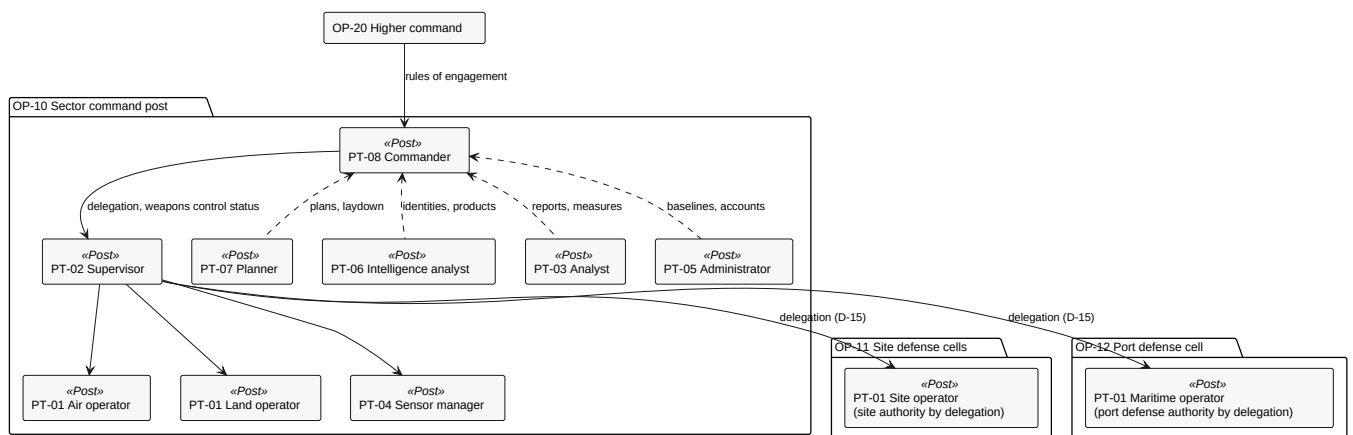
Pr-Sr: personnel structure -- the eight roles and the SecurityOfficer variant
