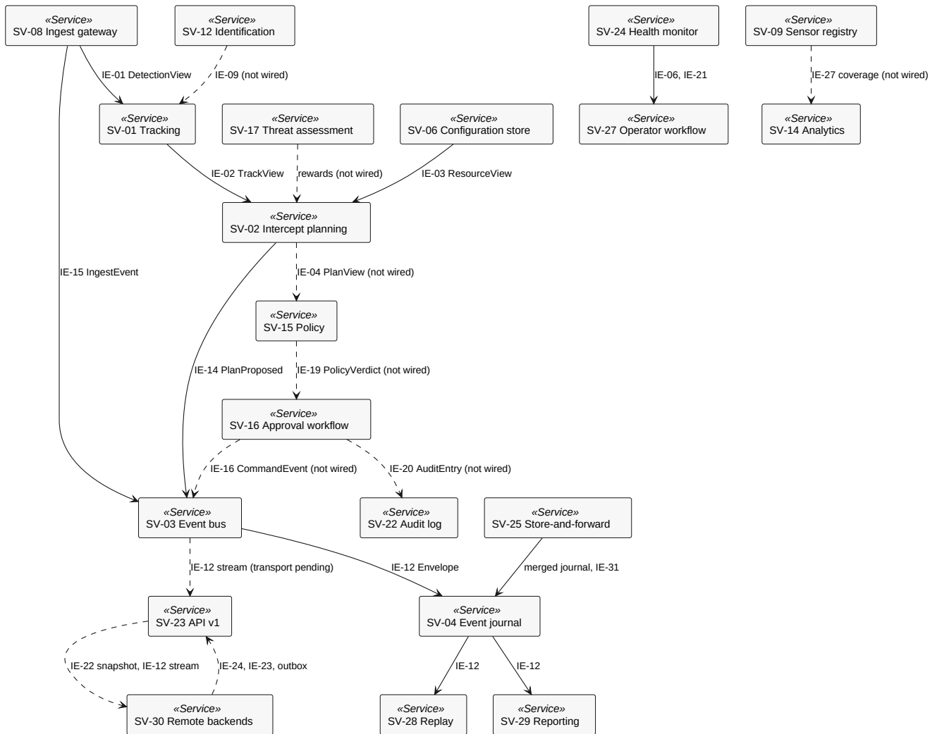
Sv-Cn: service connectivity -- information flow on one tick and across the API
