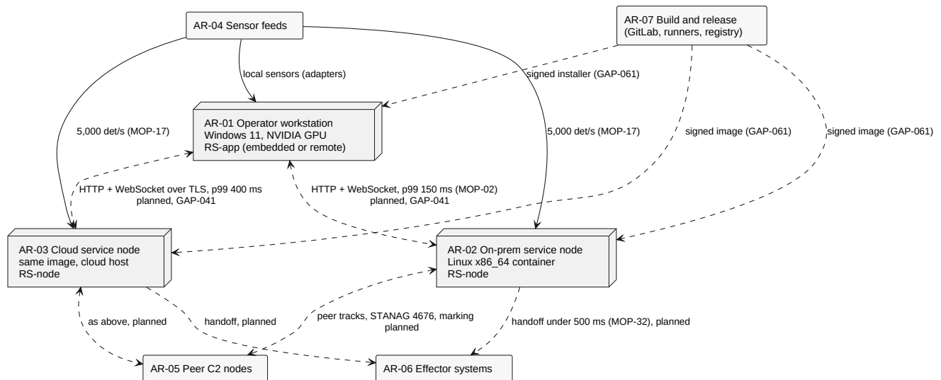
Ar-Cn: actual-resources connectivity -- the fielded instances behind the resource catalogue
