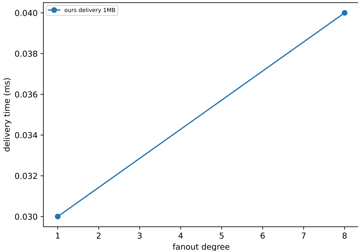
Zero-copy delivery vs fanout (flat = O(1) one-to-many)
