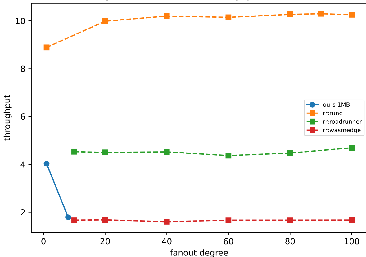
Image-resize / fanout — throughput vs fanout
