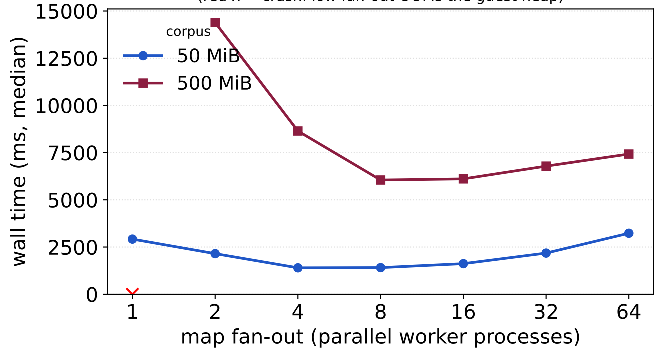
Map fan-out sweep — wall time vs worker count (red x = crash: low fan-out OOMs the guest heap)
