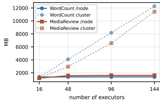
Weak — peak memory
