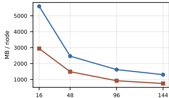
Weak — peak memory
