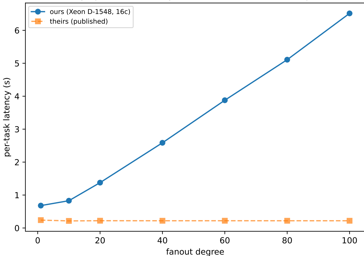
Wasmedge per-task latency — our HW vs Roadrunner published
