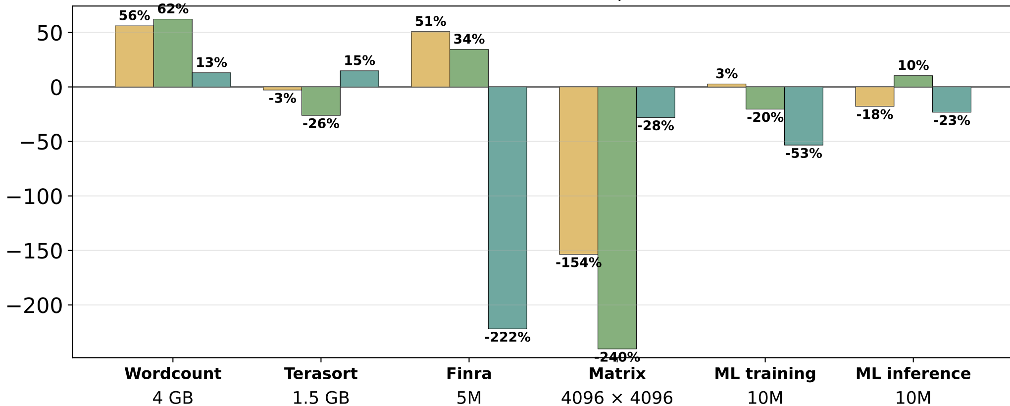
Memory saved by WasMem (%)
