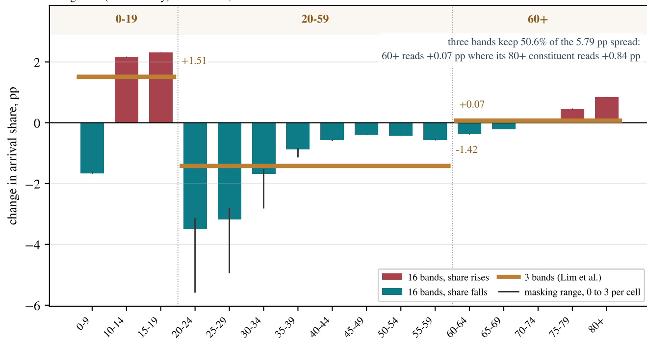
(c) age scale: the 16 published bands against the three of Lim et al., change in E (discretionary) arrival share, Dec vs Mar 2020
