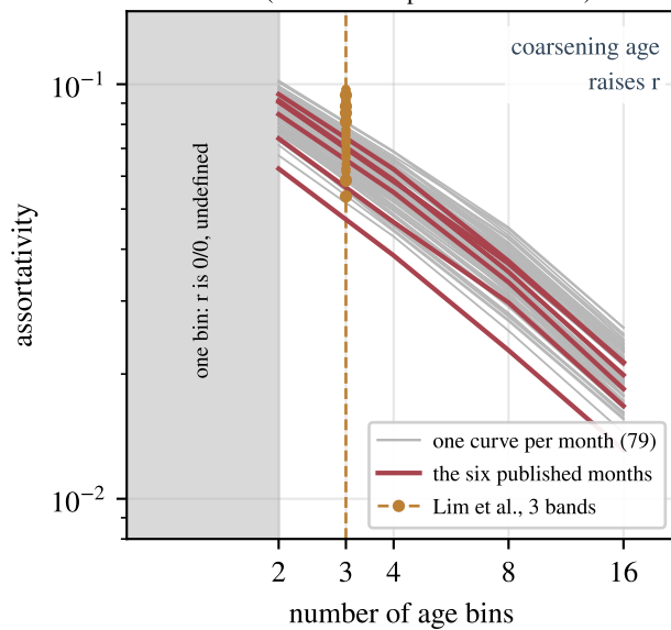
(b) age scale: the same 79 matrices, nested ladder (red = the six published months)
