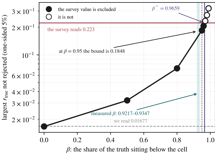
(b) the survey is excluded at every measured \beta
