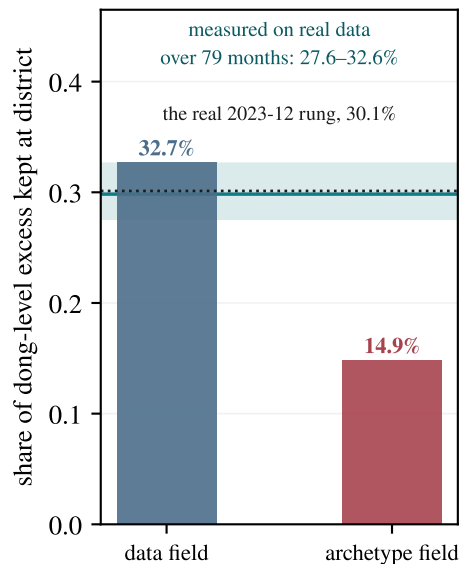
(c) an out-of-sample check
