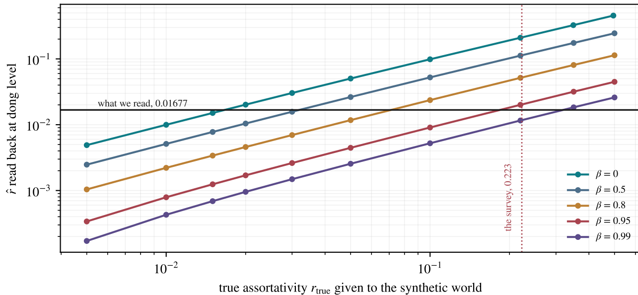
(a) what the estimator recovers
