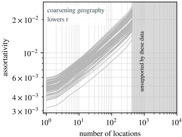
(a) spatial scale: 79 monthly curves, adjacency merge arm
