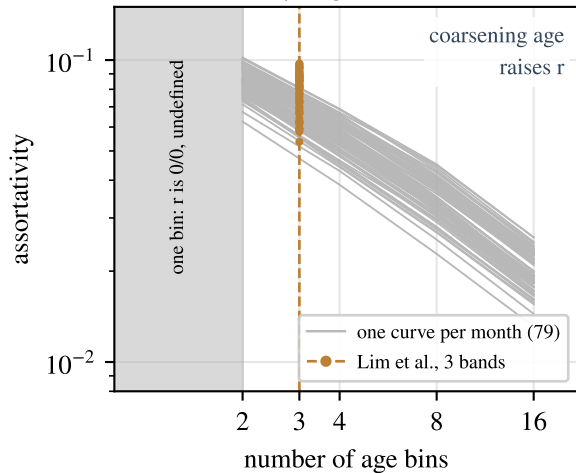
(b) age scale: the same 79 matrices, nested ladder, every rung coarsens the one above
