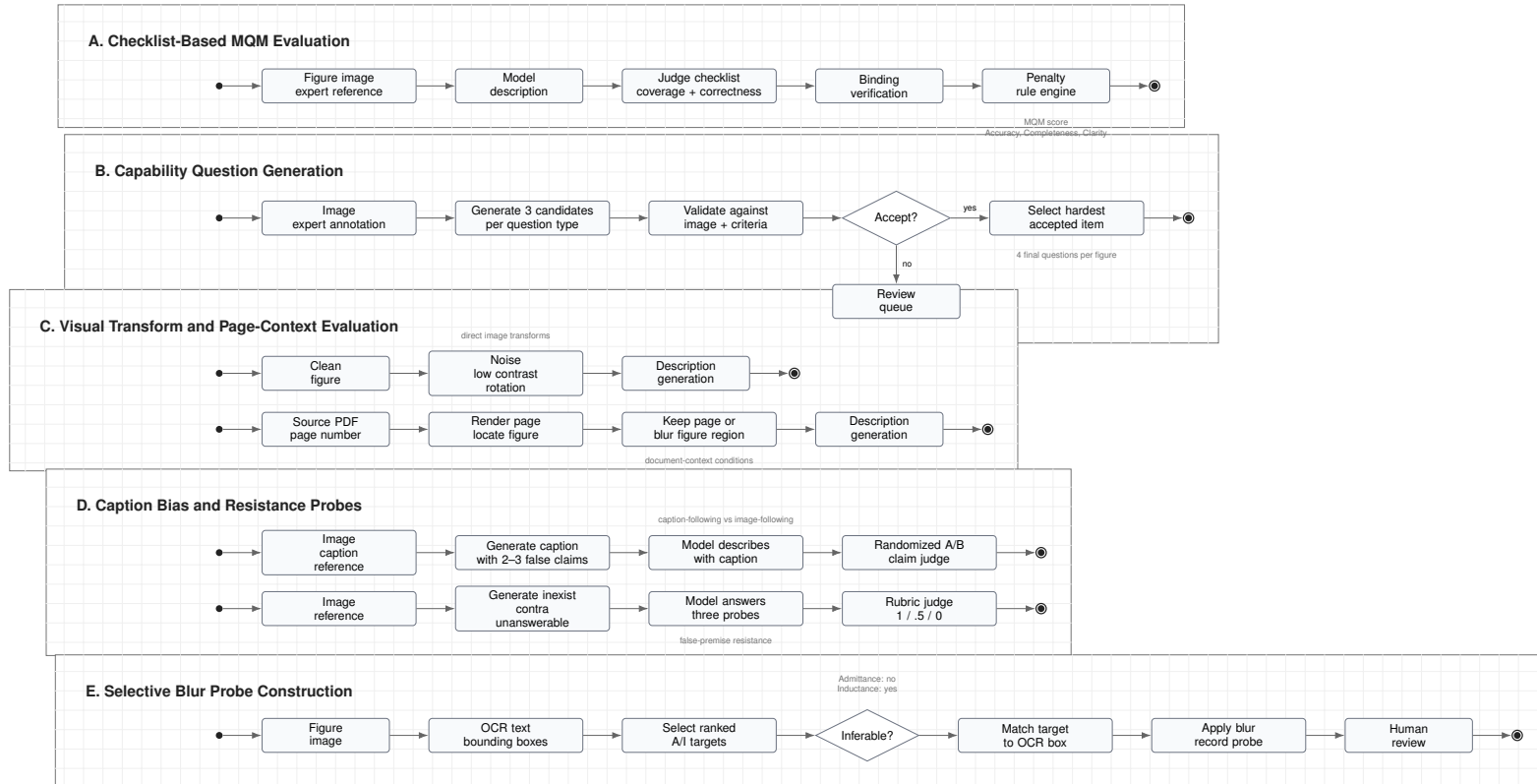
Figure 6: UML-style activity overview of the benchmark pipelines. Each panel shows the inputs, model or generator call, deterministic post-processing, and final evaluation output for one component of the benchmark.
