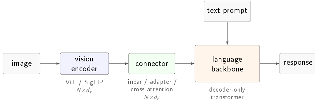
Figure 2.1: The canonical vision-language skeleton shared by every family evaluated in this thesis. A vision encoder, typically a Vision Transformer (Dosovitskiy et al., 2021) or a contrastively trained variant such as SigLIP (Zhai et al., 2023), maps the image to N patch embeddings of width d_v ; a connector (a linear projection, a lightweight adapter or a cross-attention layer) retunes them to the backbone width d_l (Liu et al., 2023); the decoder-only language model consumes them as a prefix alongside the text prompt. Families differ in how each stage is realised, not in the skeleton itself.
