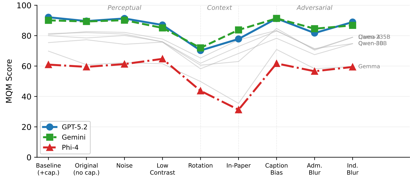
MQM across evaluation conditions
