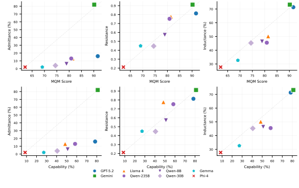
Figure 4: Quality does not predict behaviour. Each model is plotted by its MQM description quality (x-axis) against admittance rate (left) and resistance score (right). The dashed line shows where points would fall if quality predicted behaviour. GPT-5.2 (blue) and Gemini (green) score comparably on quality but diverge sharply on both behavioural dimensions. Phi-4 (red) is low on all axes.
