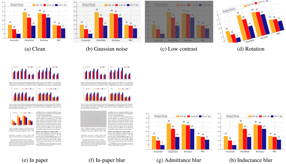
Figure 5: Representative visual conditions for Figure 042. The first row shows the clean figure and direct perceptual transformations. The second row shows document-context and selective-blur conditions. Admittance blur removes information intended to be unrecoverable; inductance blur removes information selected to remain inferable from context.
