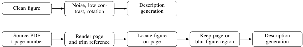
Figure 8: Pipelines for visual transformations and page-context conditions. Direct transforms alter the isolated figure; page-context conditions render the source PDF page and optionally blur the target figure region.
