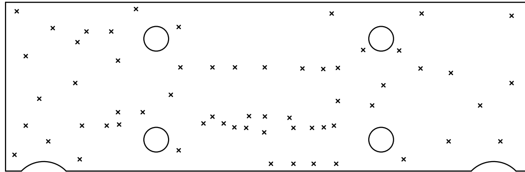
Drill Map: x 0.300mm / 0.0118" (61 holes)
