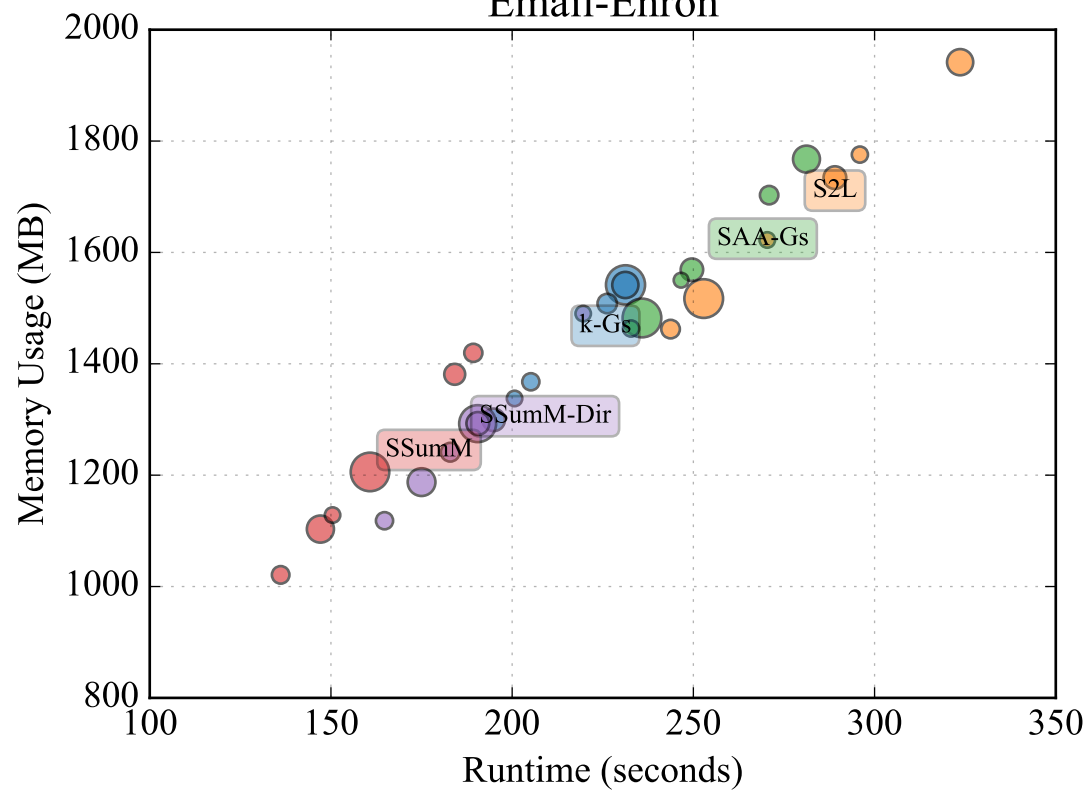
Email-Enron
