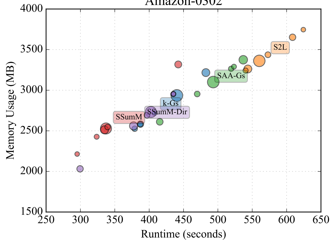
Amazon-0302
