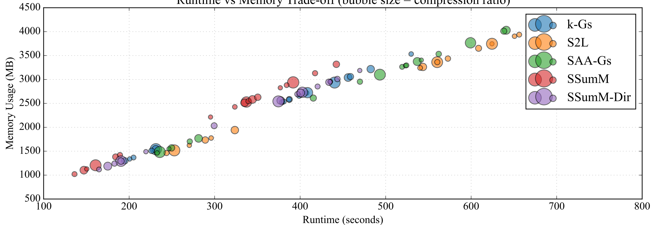
Runtime vs Memory Trade-off (bubble size = compression ratio)
