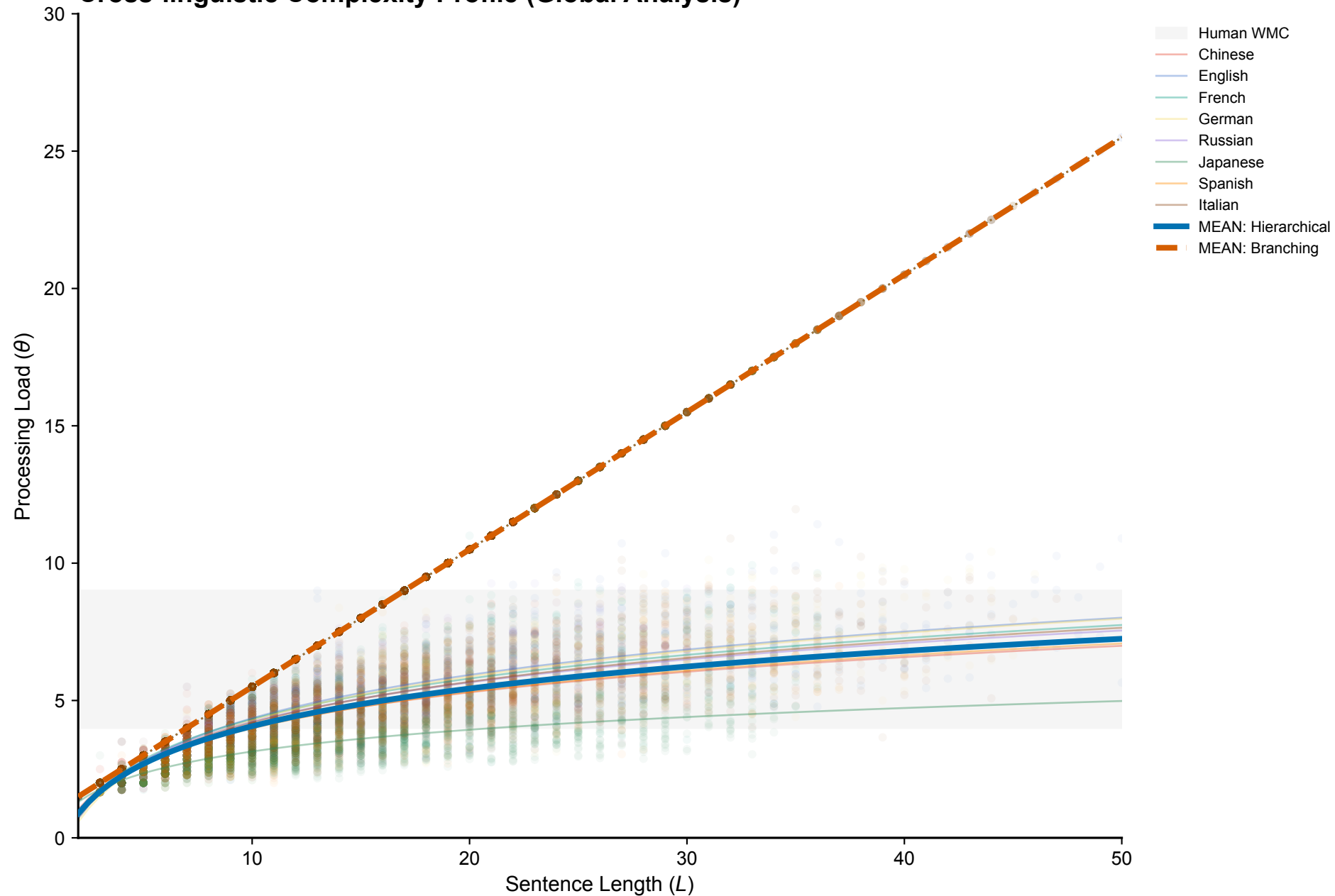
Cross-linguistic Complexity Profile (Global Analysis)
