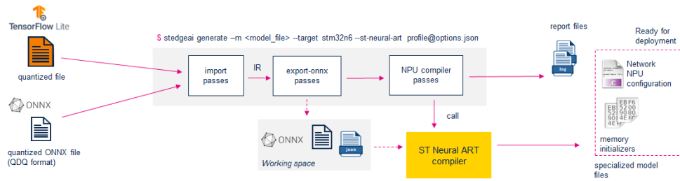
Abbildung 2.7.: NPU – Quantized Model Conversion to NPU Executables [35]
