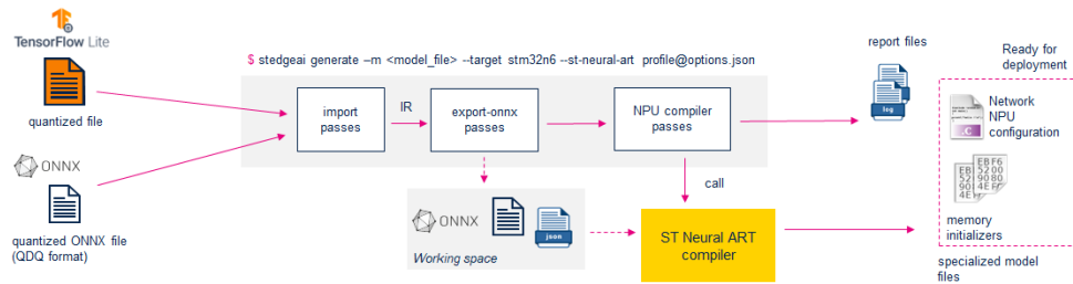
Abbildung 2.7.: NPU – Quantized Model Conversion to NPU Executables [32]
