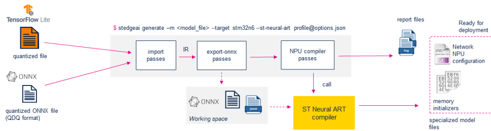
Abbildung 2.7.: NPU – Quantized Model Conversion to NPU Executables — (ST Neural-ART NPU – Supported Operators and Limitations, n.d.; ST Neural-ART NPU Concepts, n.d.)
