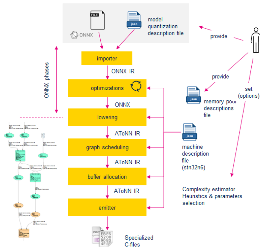
Abbildung 2.8.: NPU – Compilation — (ST Neural-ART NPU – Supported Operators and Limitations, n.d.; ST Neural-ART NPU Concepts, n.d.)
