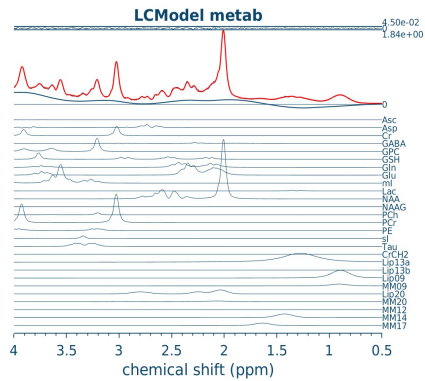
Figure 3. MRS data quality A) Average MRS location. Colored overlay of the average voxel location across all nineteen participants, from 0 (black) to 1 (white). Brighter yellow represents voxel locations shared by all participants, while darker purple represents voxel locations unique to participants. MRS voxels were registered to MNI space and averaged. Underlay is T1w MNI152 at 0.5 mm resolution. B) Sample Osprey sLASER Spectrum. Red spectrum indicates overall model fit. Model fits for individual metabolites are shown in blue below overall fit. C) Sample Osprey MEGA-PRESS Spectrum. Yellow spectrum indicates overall model fit. Model fits for individual metabolites are shown in blue below overall fit.
