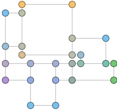
Vertex Graph
