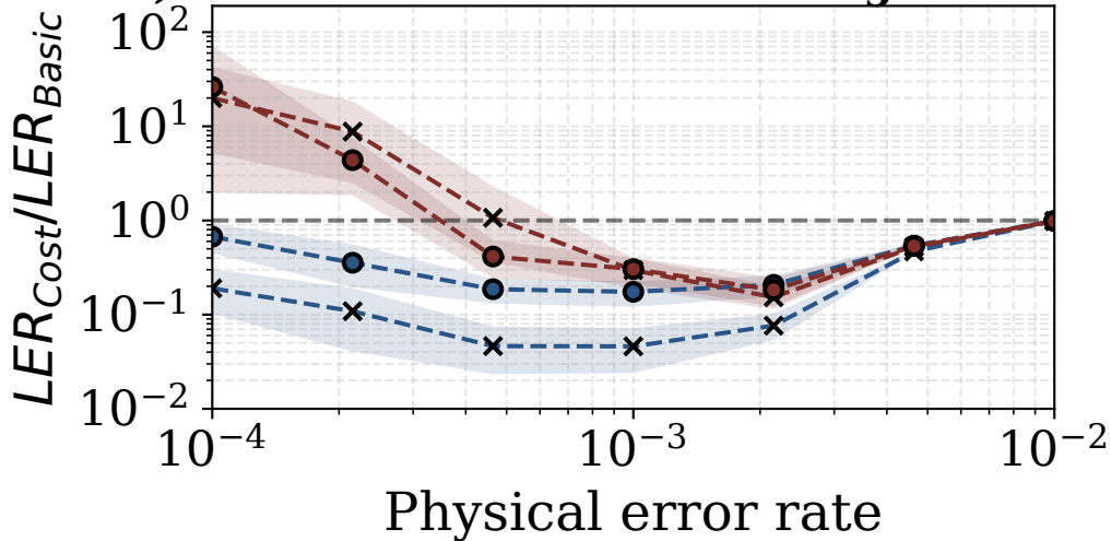
c) Relative effect of cost-routing on LER
