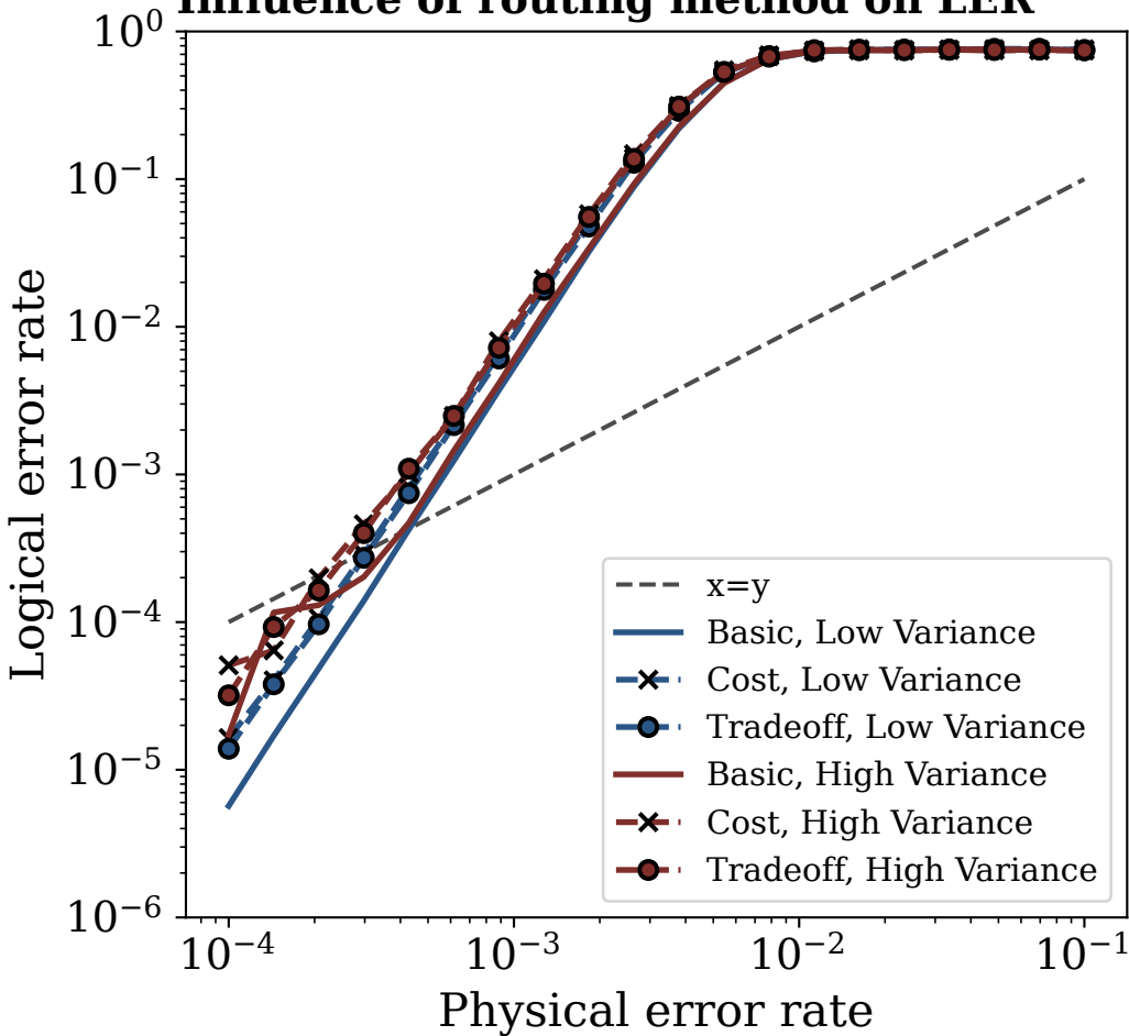
Influence of routing method on LER
