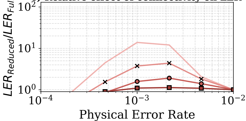
c) Relative effect of connectivity on LER
