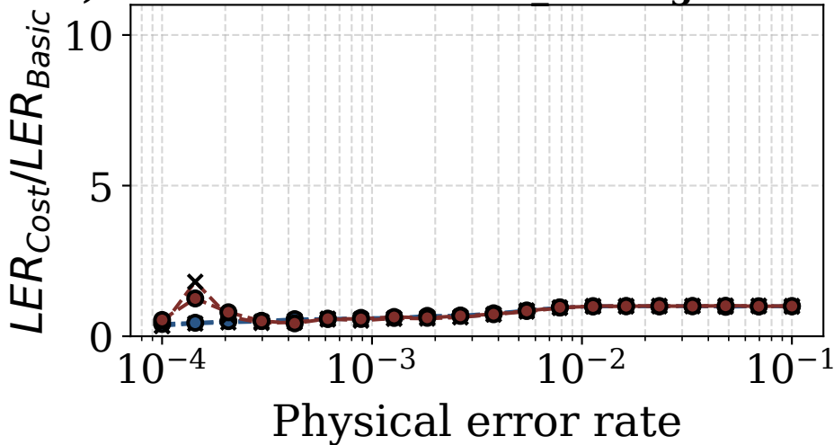
c) Relative effect of cost_routing on LER
