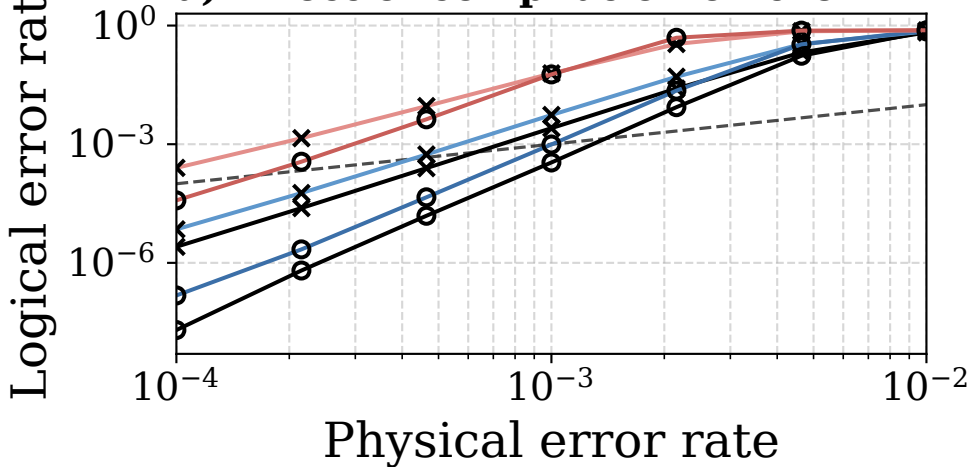
Lower is better ↓ a) Effect of compilation on the LER
