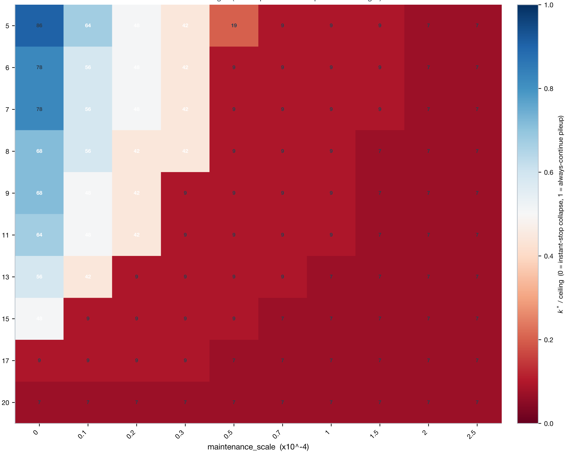
REGIME sweep: SingleHalt*'s own k^* (cell text) across cost regimes hatched = NOT meaningful ( k^* collapsed to \leq 1 or pinned at ceiling-1)
