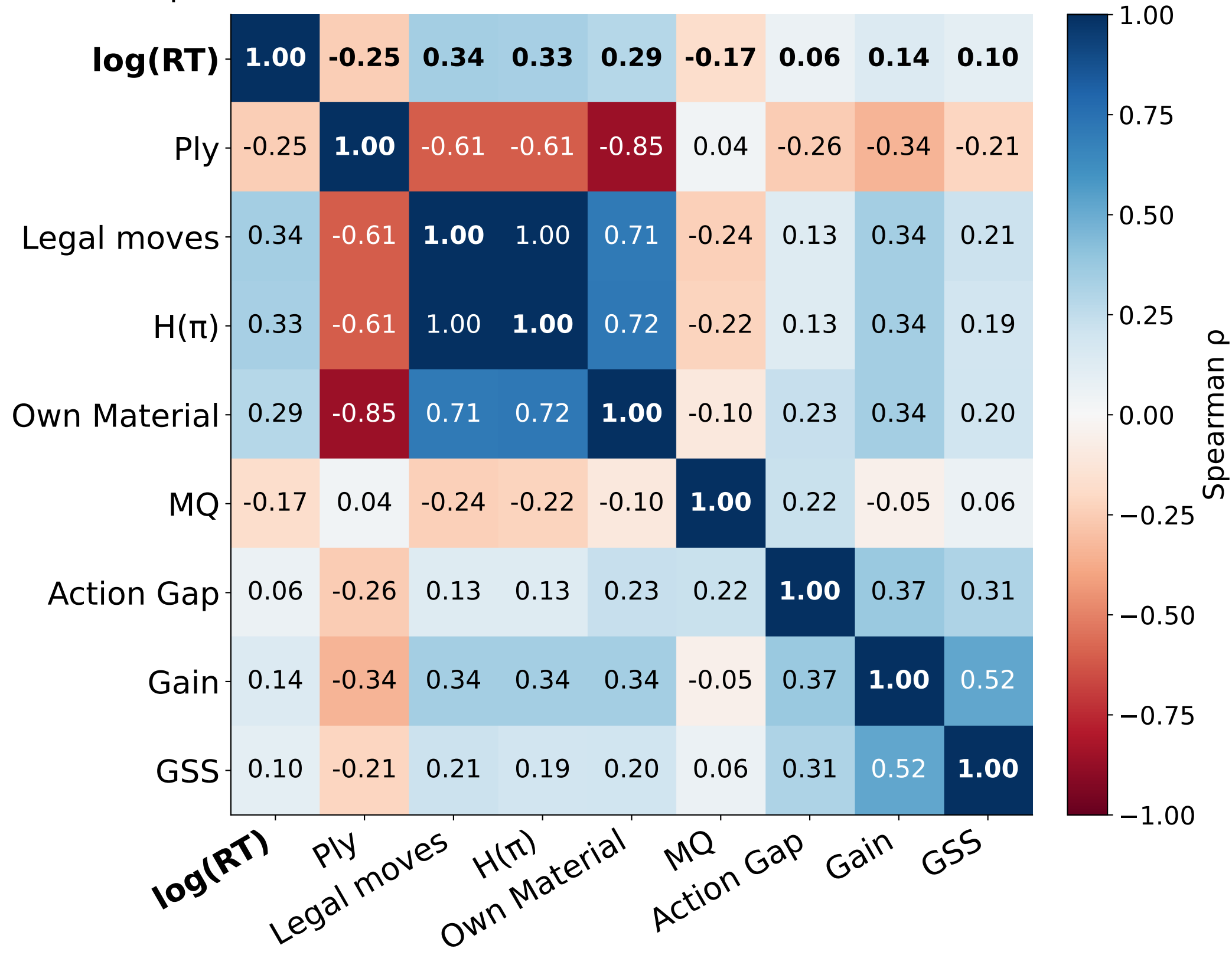
Spearman correlation — SF-1 (n1·d36) metrics (n = 105,141)
