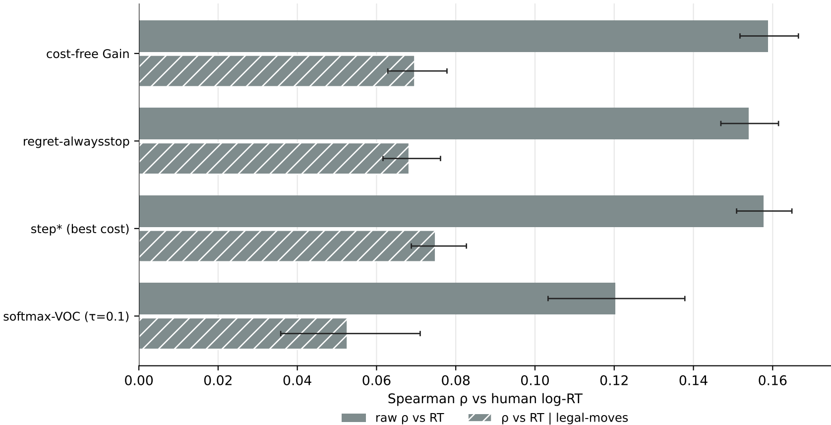
Value-of-computation signals are proxies for legal-moves (n=64,751)
