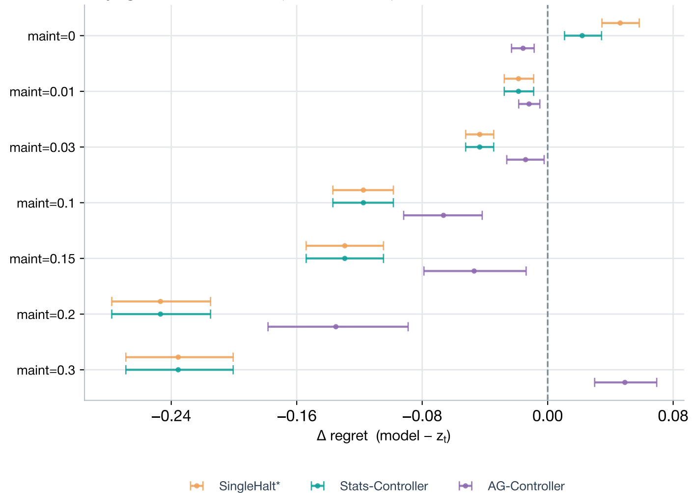
varying maintenance scale (linear \lambda=0.0015 )
