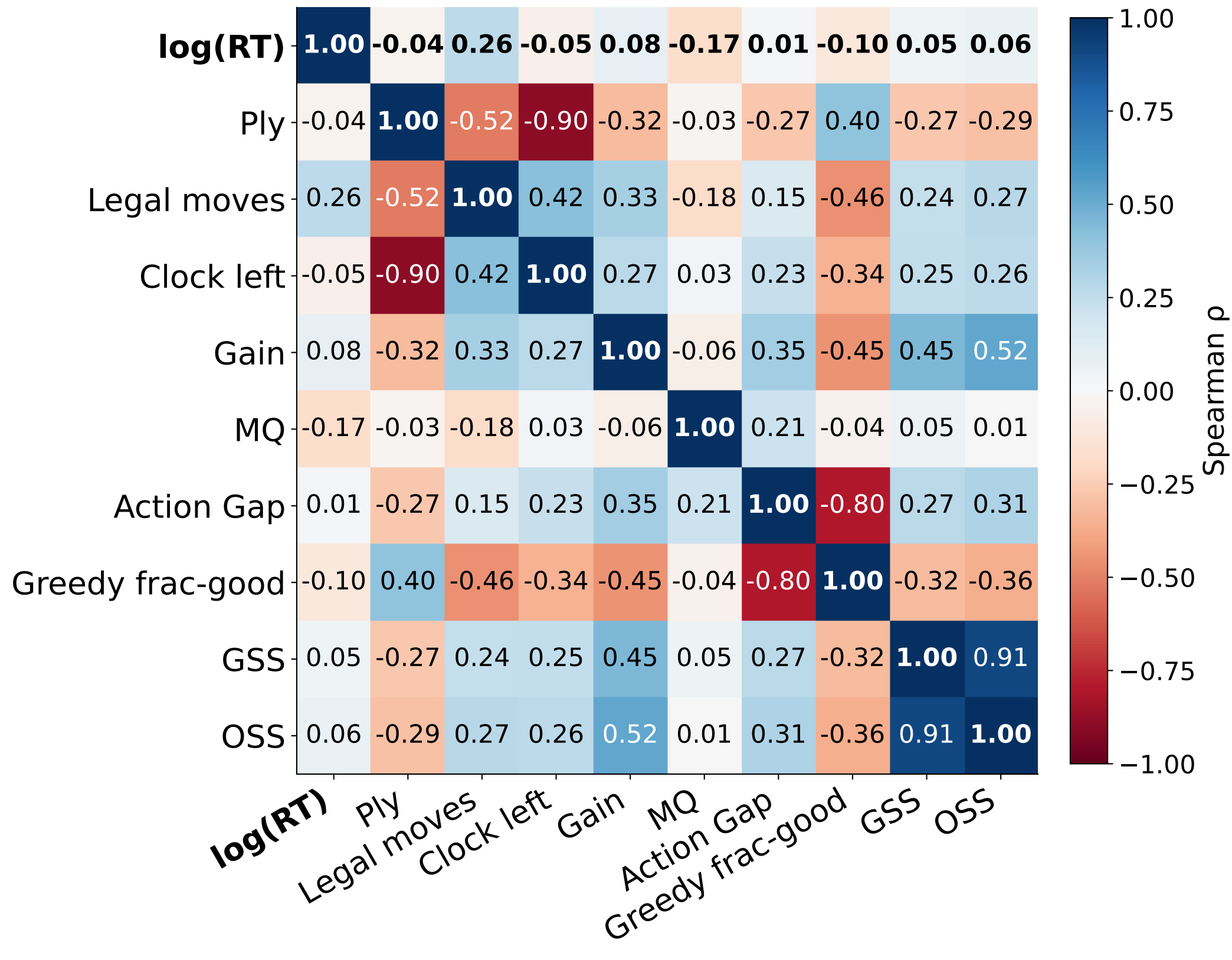
Spearman correlation — SF-1 (n1·d36) metrics (n = 109,434)
