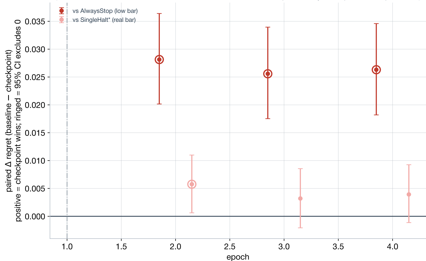
Sub-line A: paired 95% CI, regret diff vs AlwaysStop / SingleHalt* (time_lambda=0.01, maintenance_scale=0.001 -- confirmed win at epoch 2 only, not replicated at epochs 3-4)
