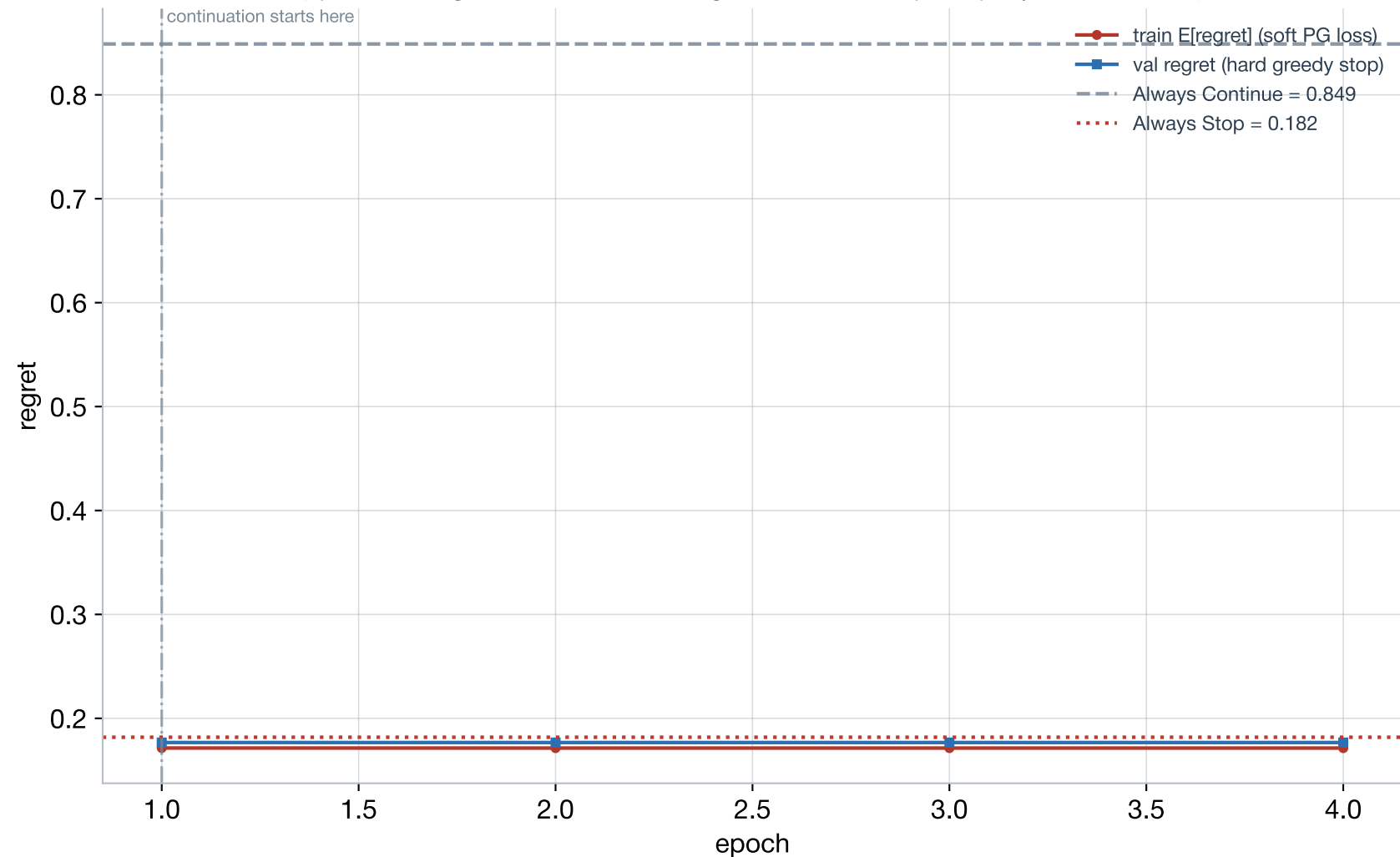
Sub-line A: e2e (encoder-unfrozen) controller, soft-loss vs epoch (epoch 1 = original Z2 run; 2+ = this agent's chained 1-epoch-per-job continuation)
