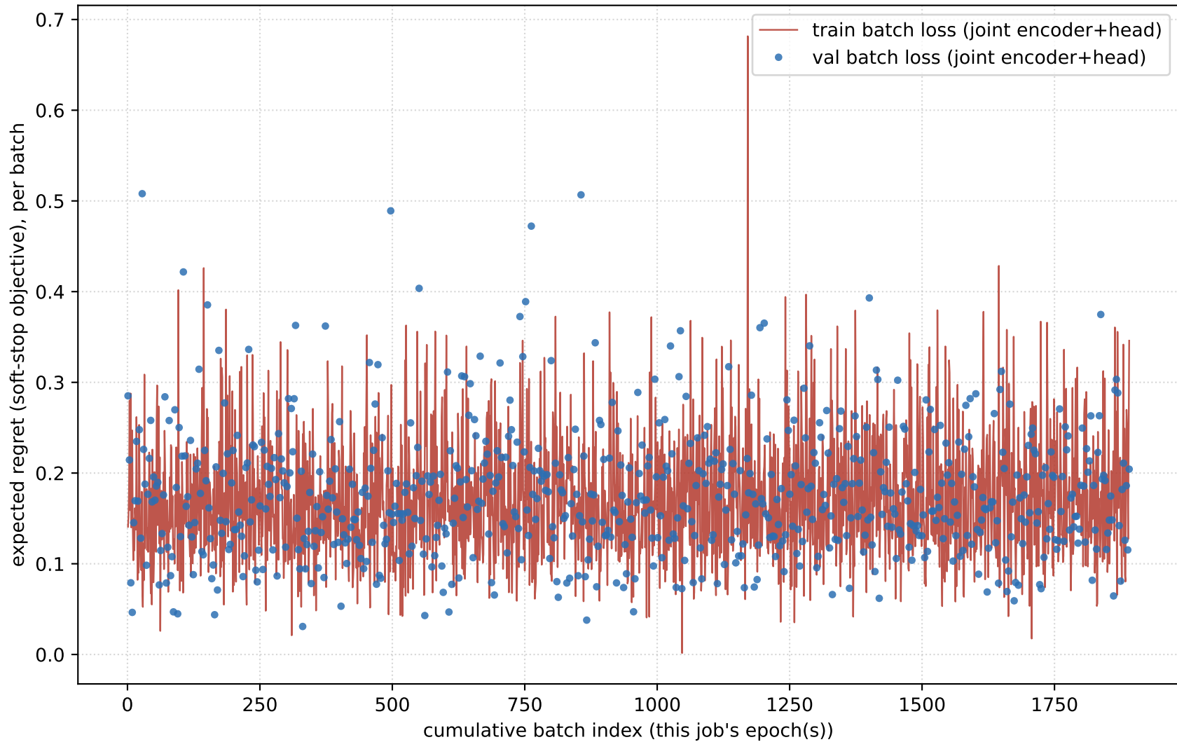
Z2/Z-EXT: within-epoch batch loss trace
